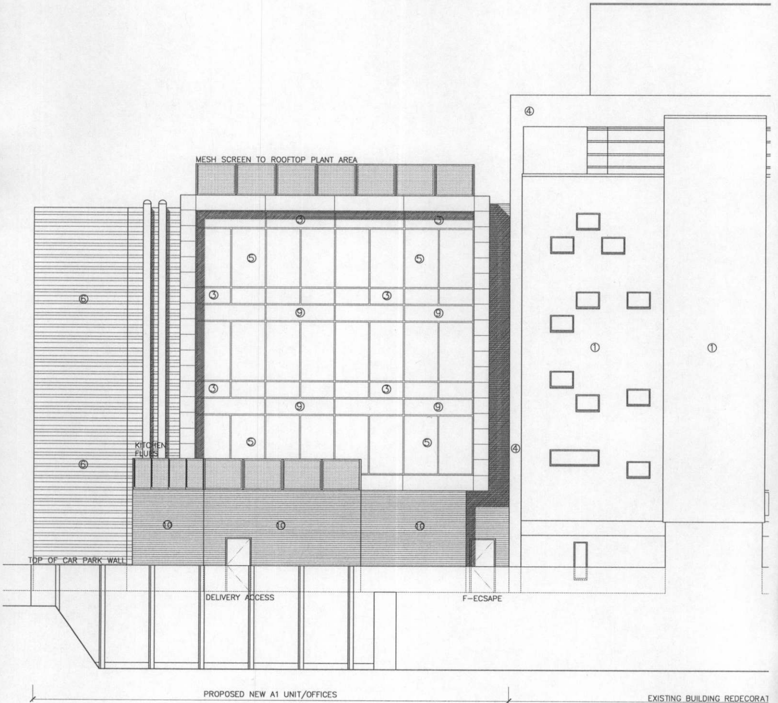
SOUTH EAST ELEVATION (CAR PARK)
