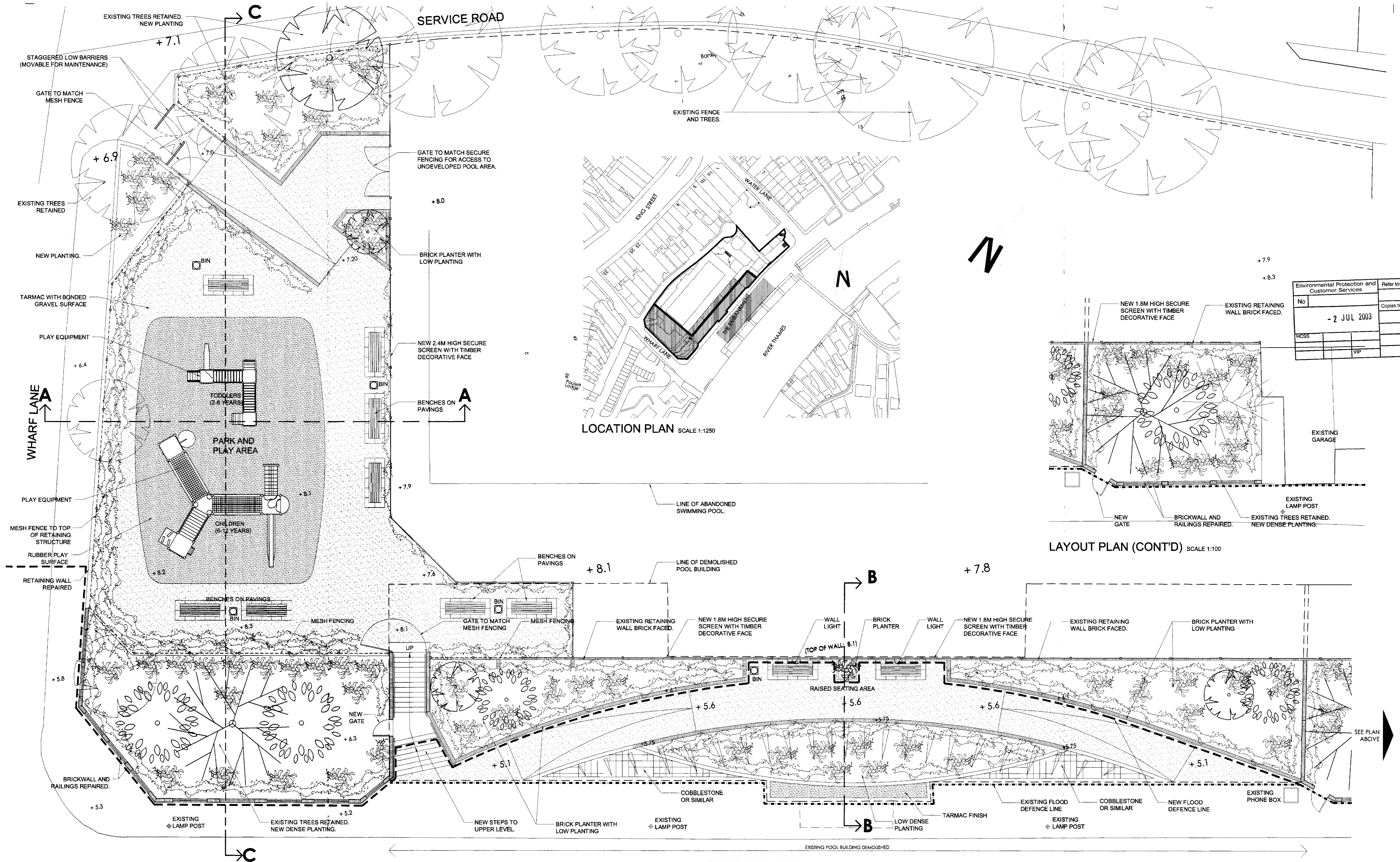
LAYOUT PLAN SCALE 1:100
