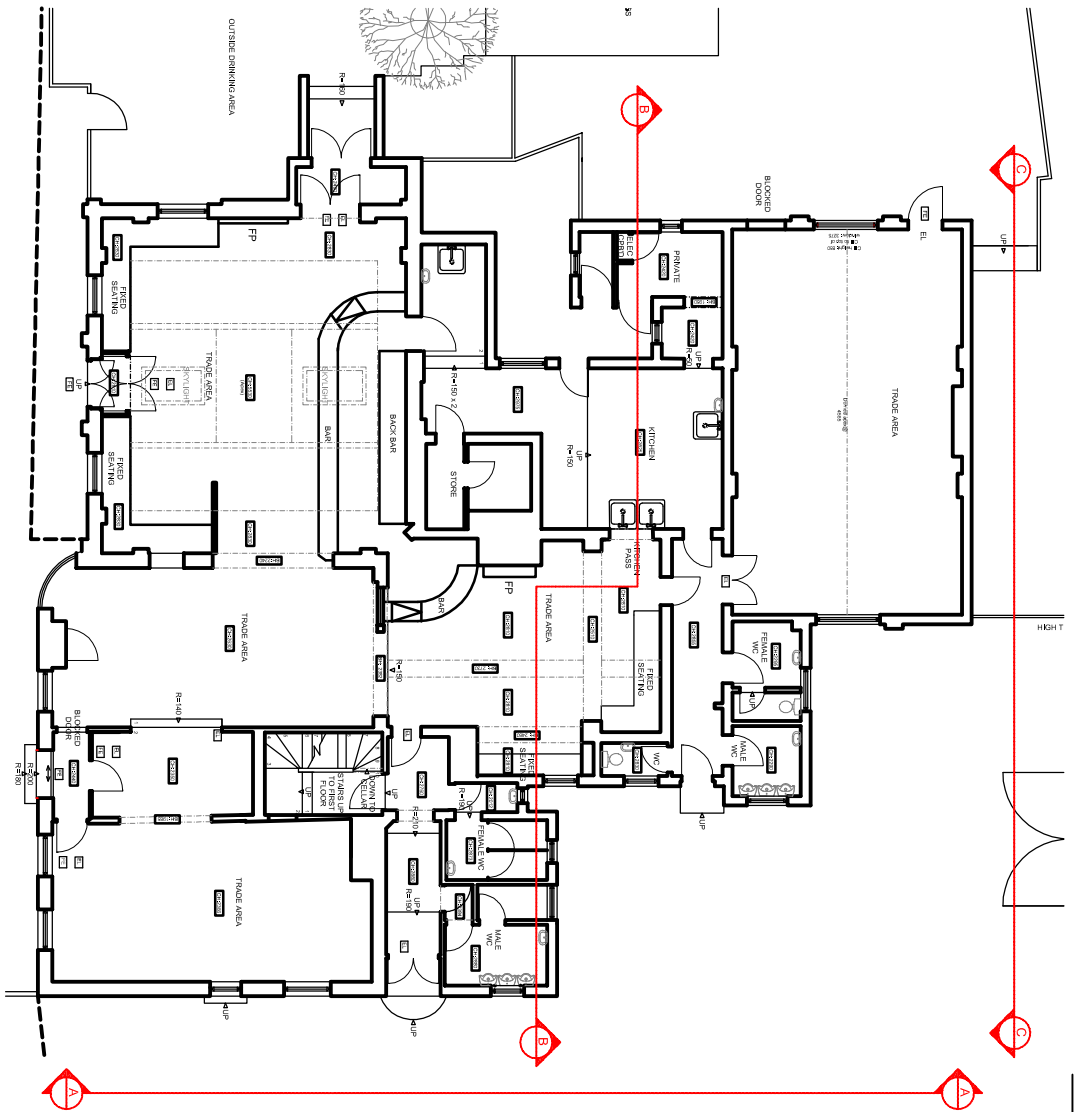
EXISTING PLAN. 1:100 @ A1
