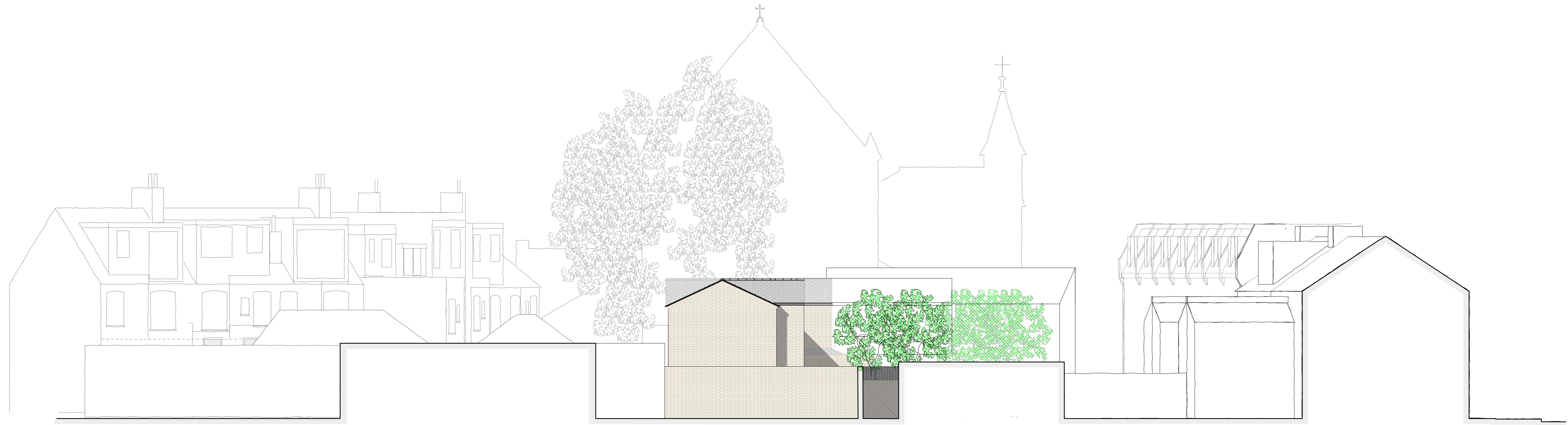
WEST ELEVATION
