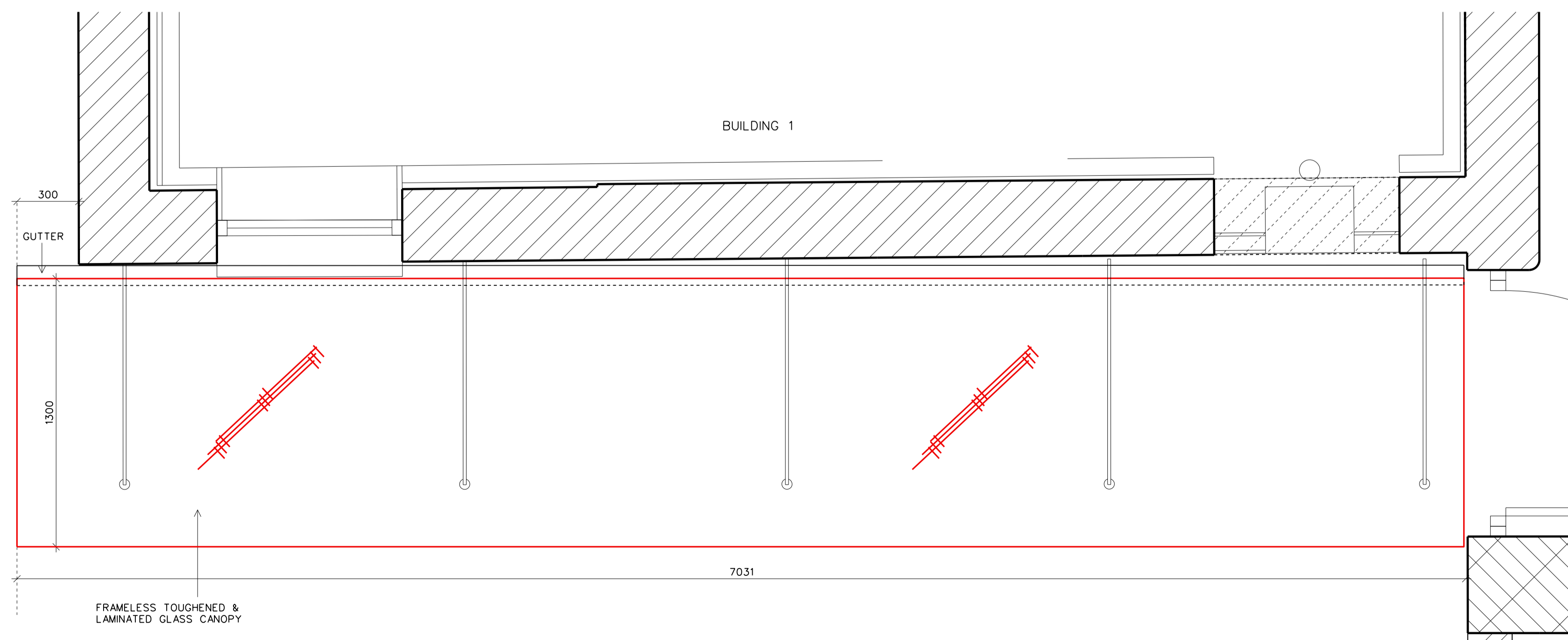
PLAN OF ENTRANCE CANOPY
