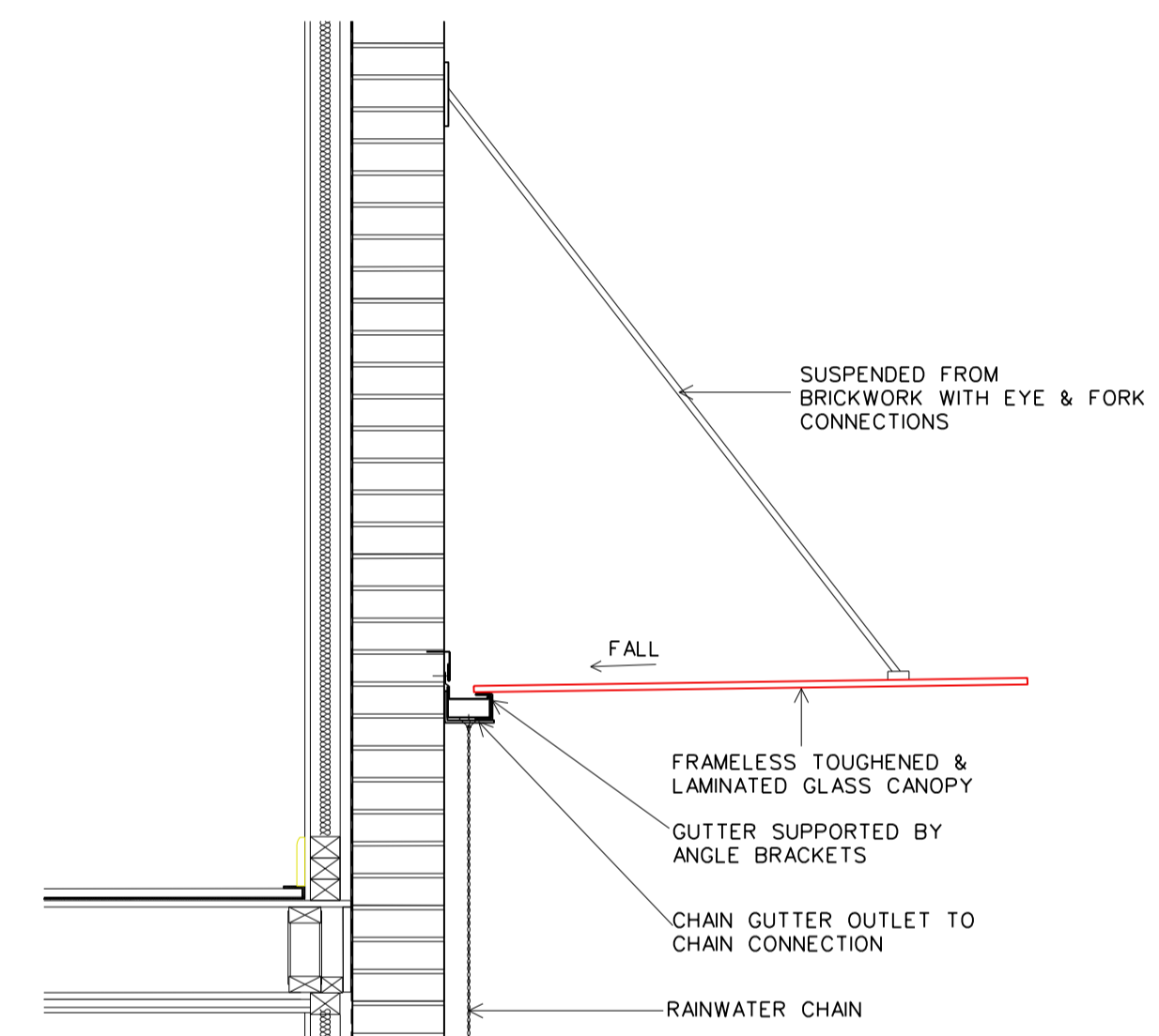
SECTION THROUGH CANOPY
