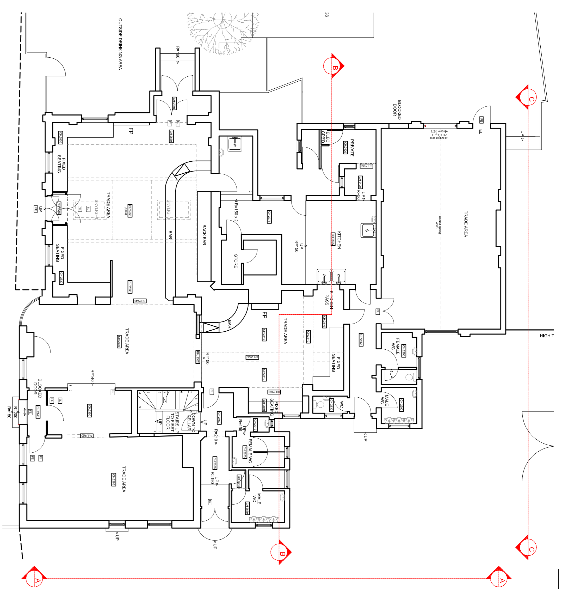
EXISTING PLAN. 1:100 @ A1
