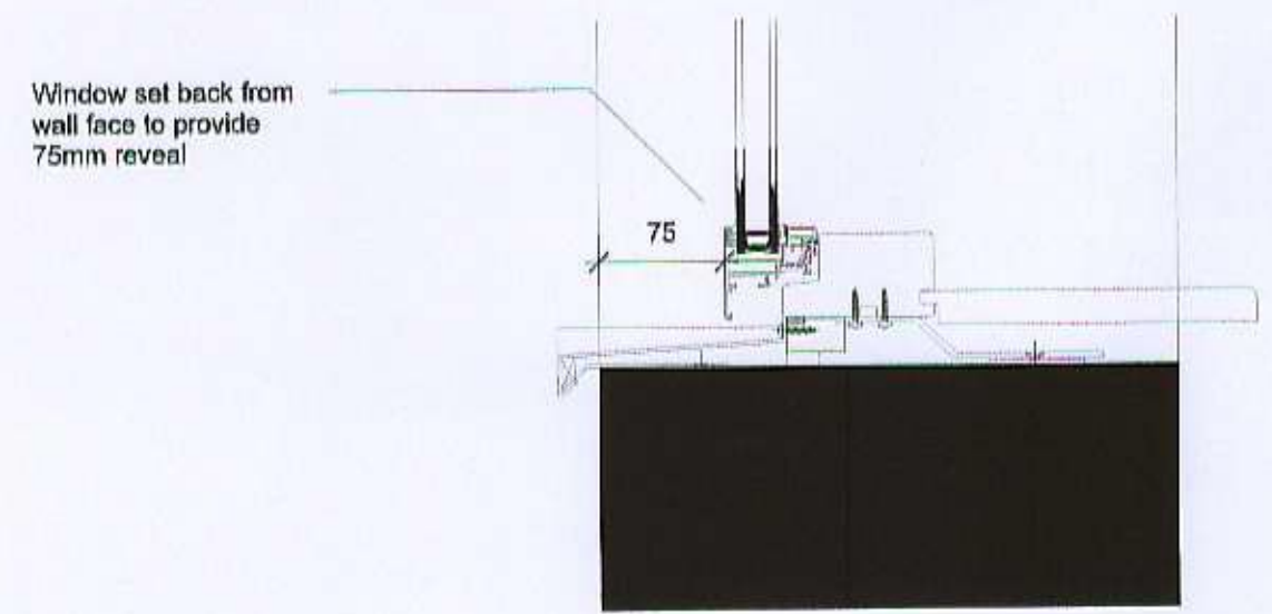
Detail 02: Window Cill 1:5 @ A1
