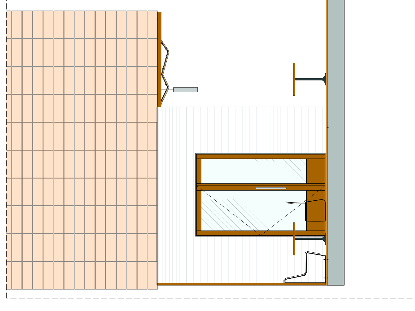
3 ELEVATION F
