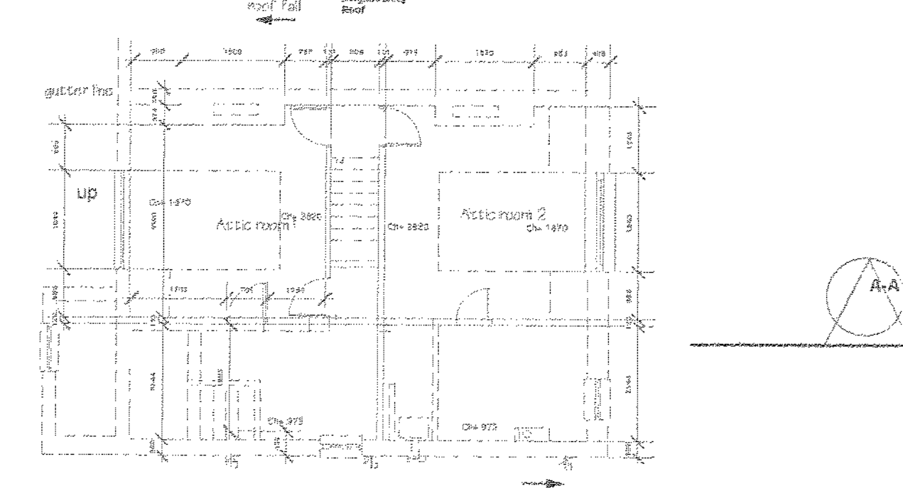
Second Floor & roof floor plan
