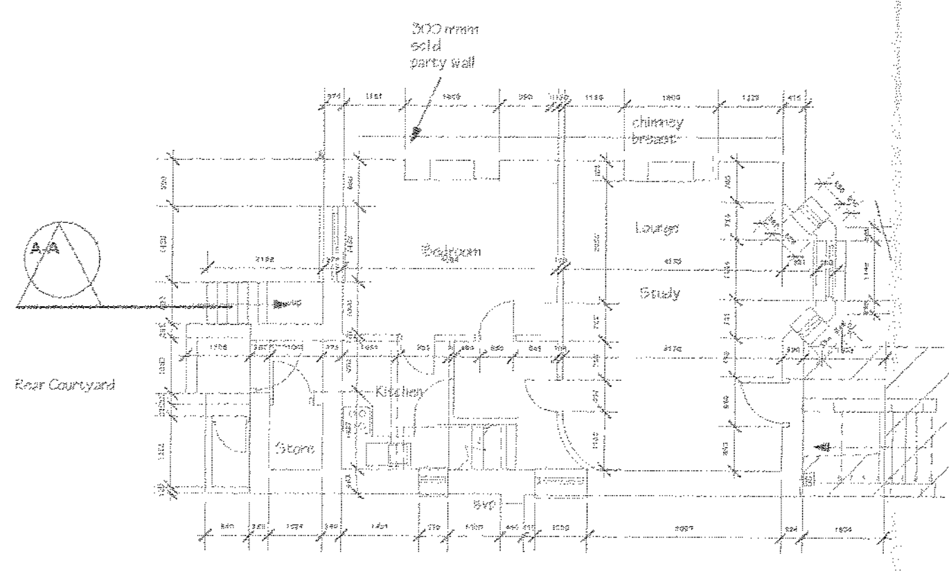
Lower ground floor plan Basement
