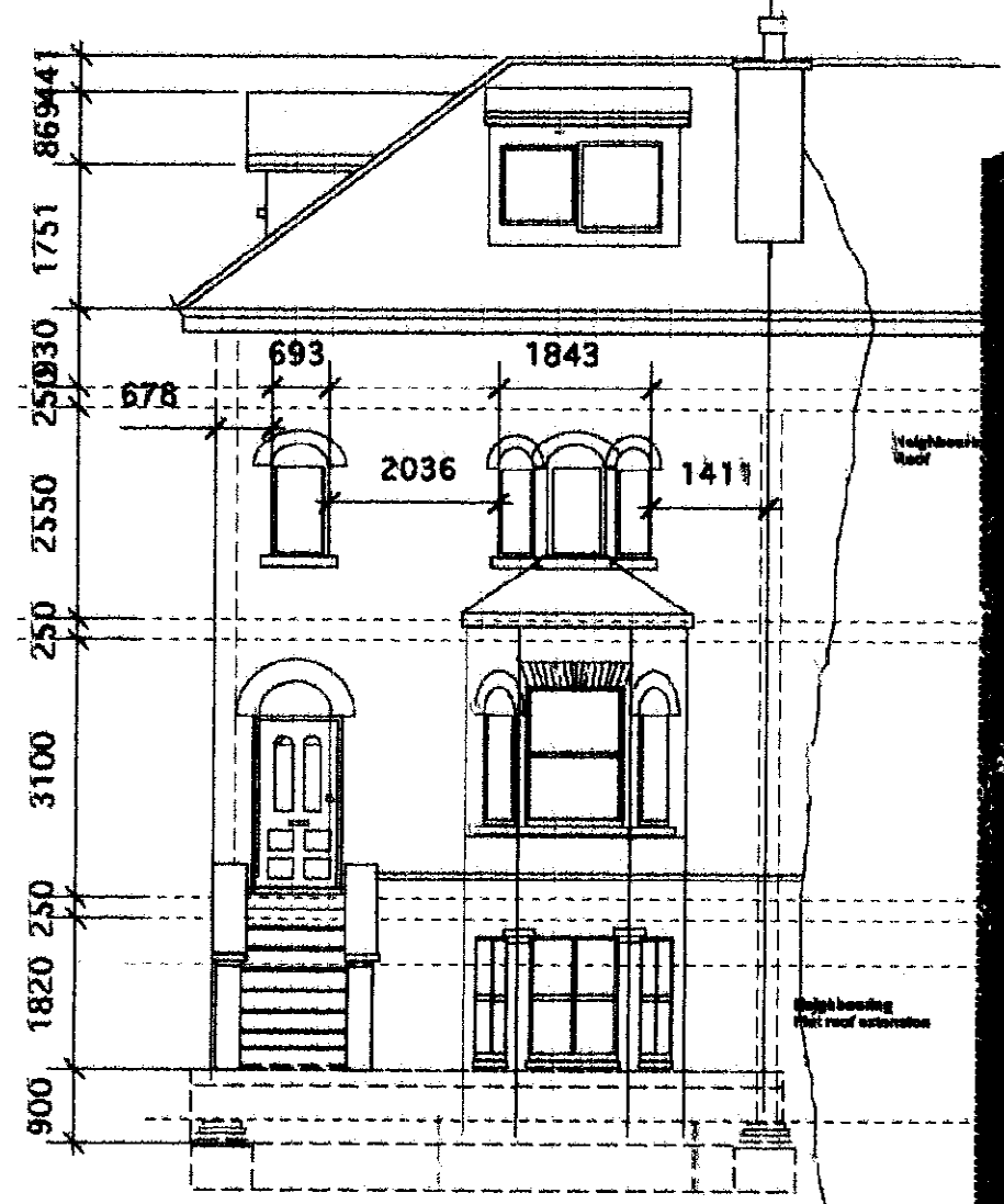
Front West Elevation
