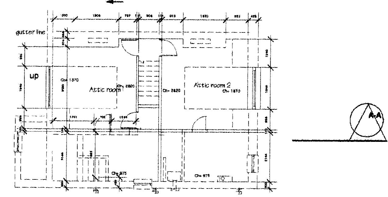
Second Floor & roof floor plan
