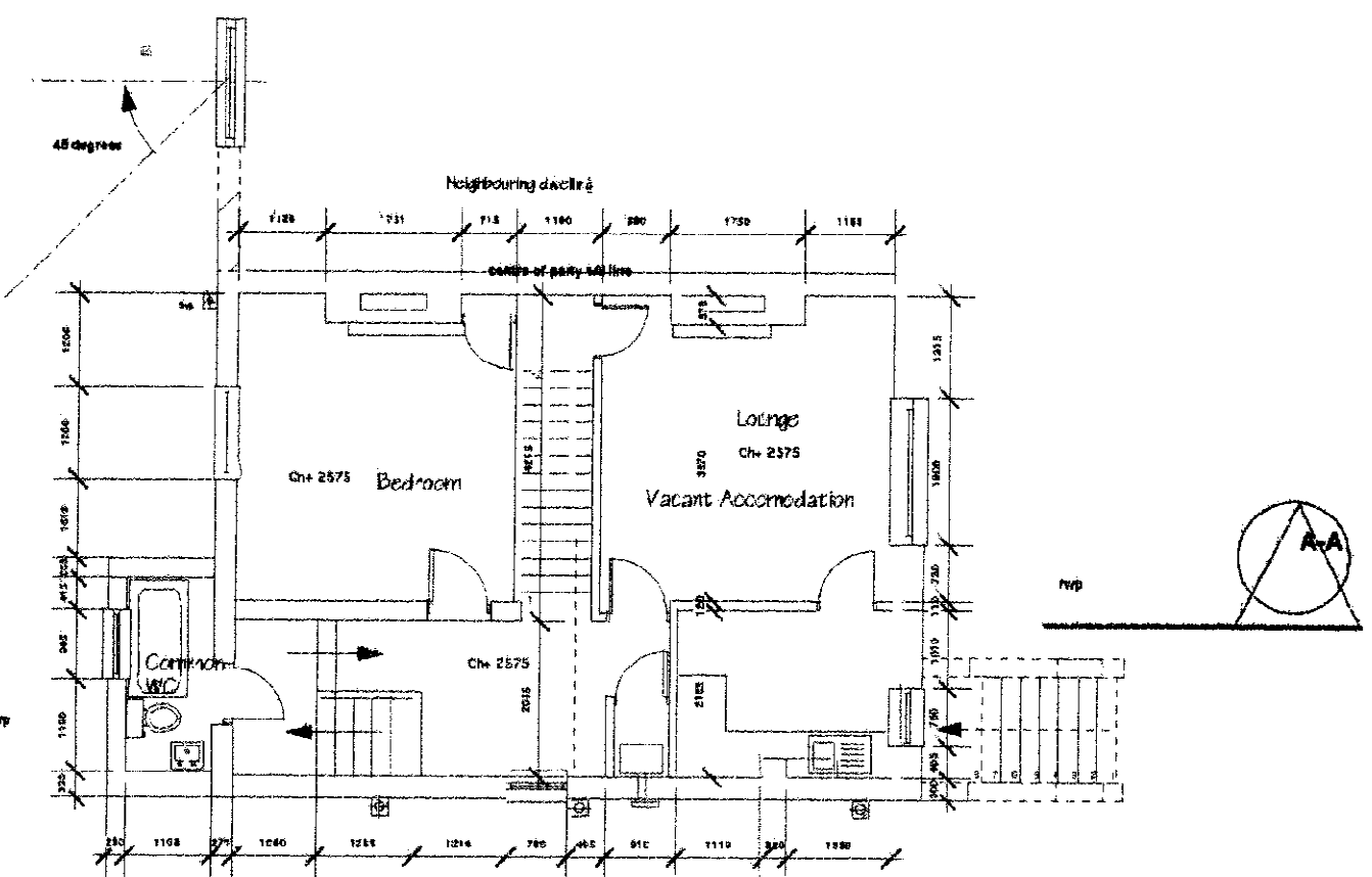
First Floor Accomodation with common WC Areas
