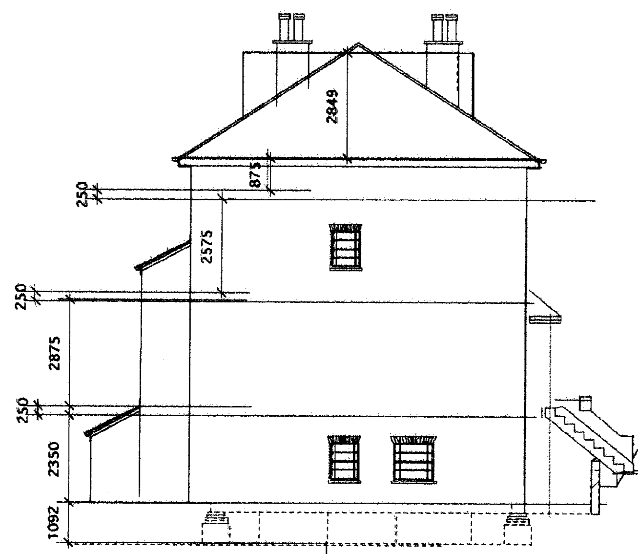
Side North Elevation
