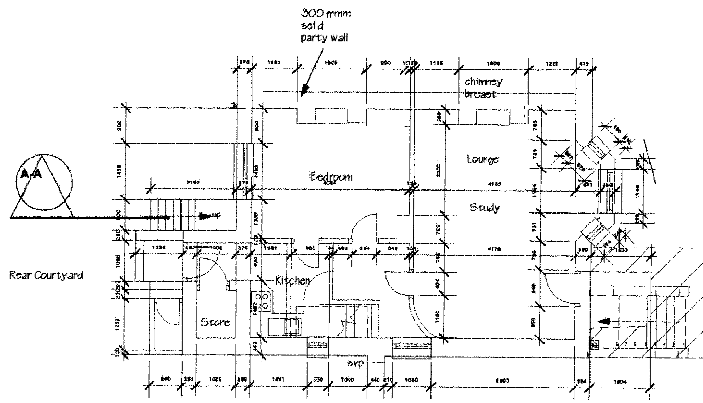
Lower ground floor plan Basement
