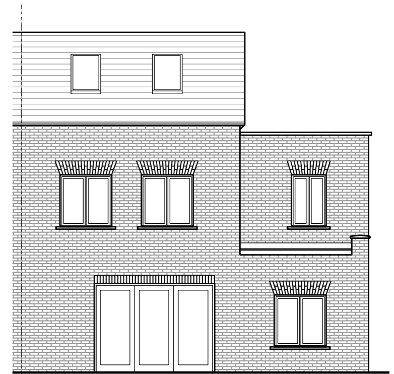
Rear Elevation House Type E2
