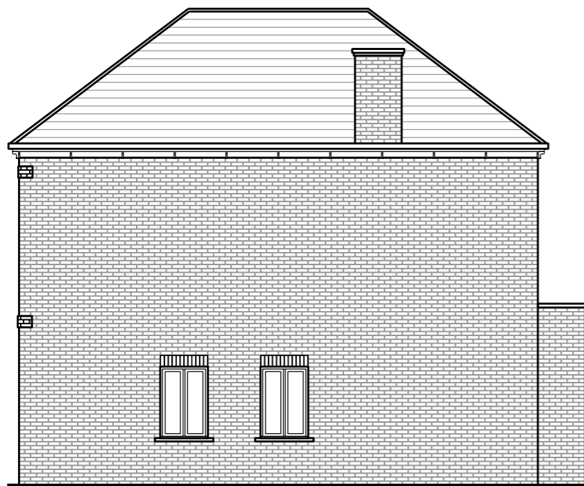
Side Elevation - House Type F2
