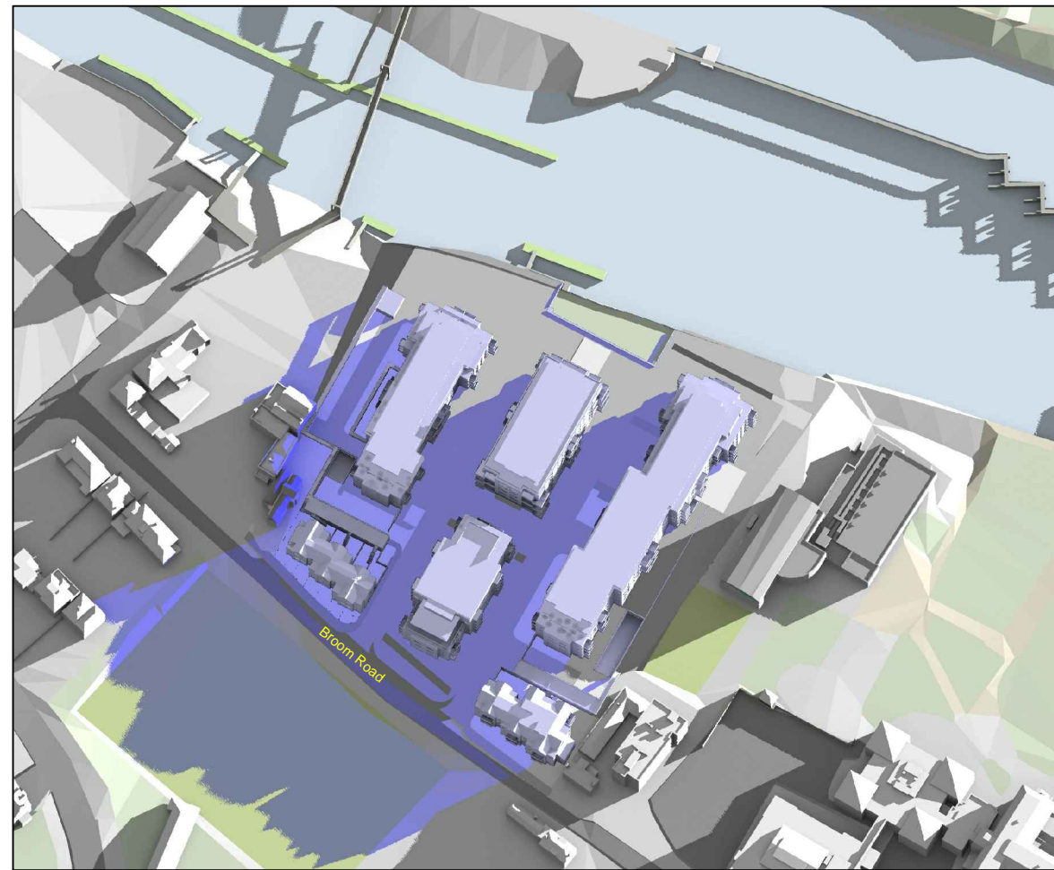
PROPOSED - 6:00am
