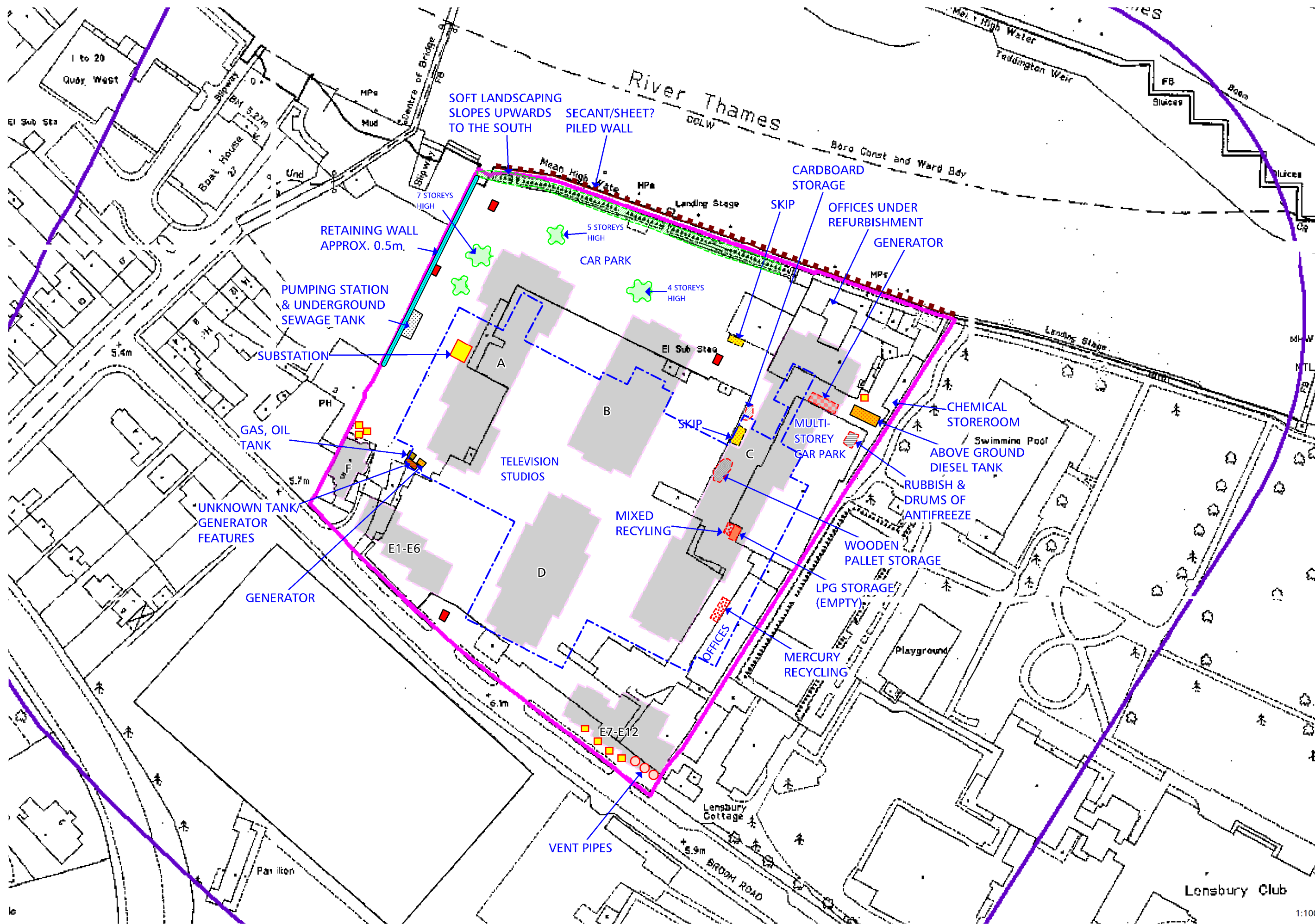
Figure 2.2: Annotated Site Layout
