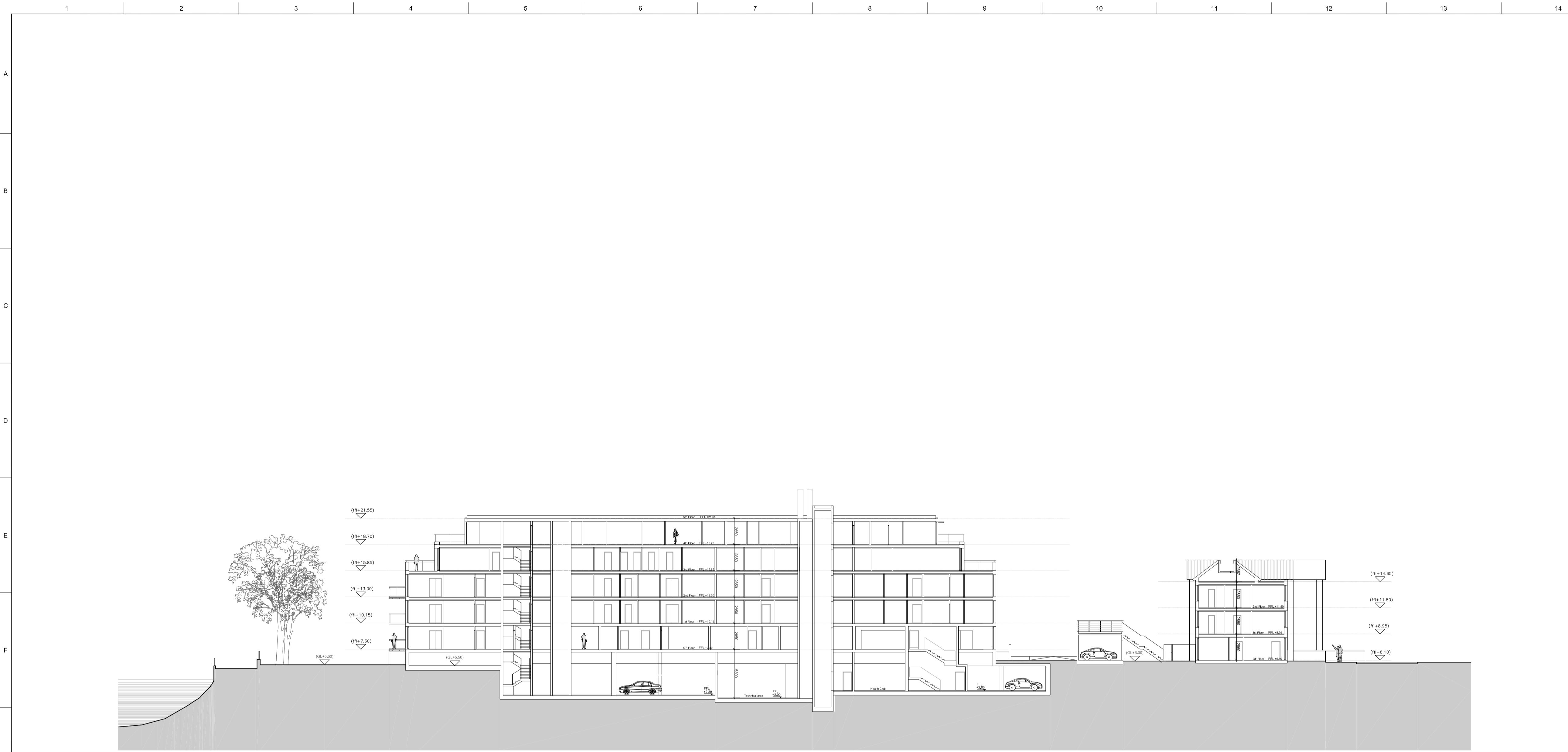
Proposed Section 1-1'
