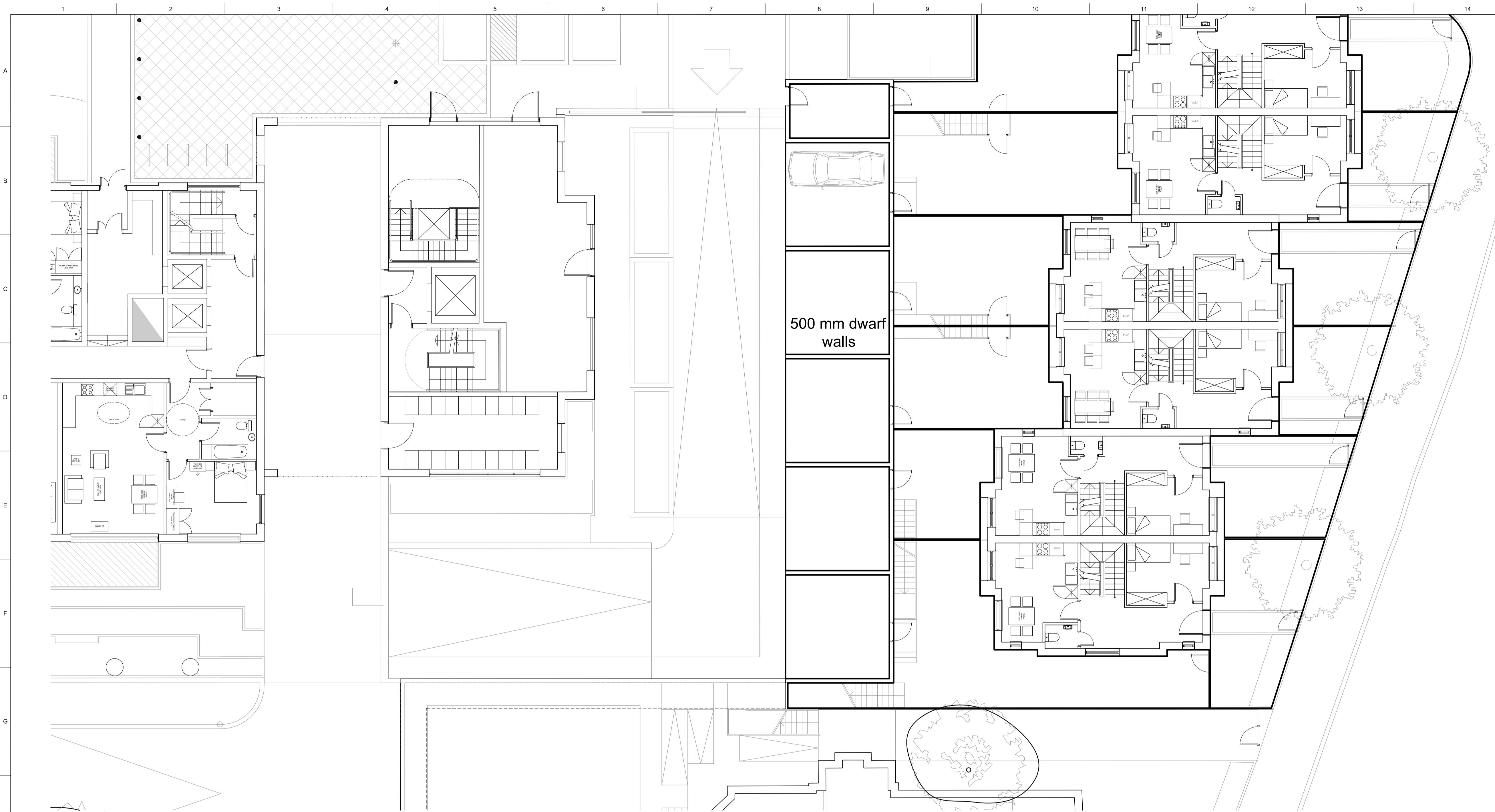
Plan detail 1:100
