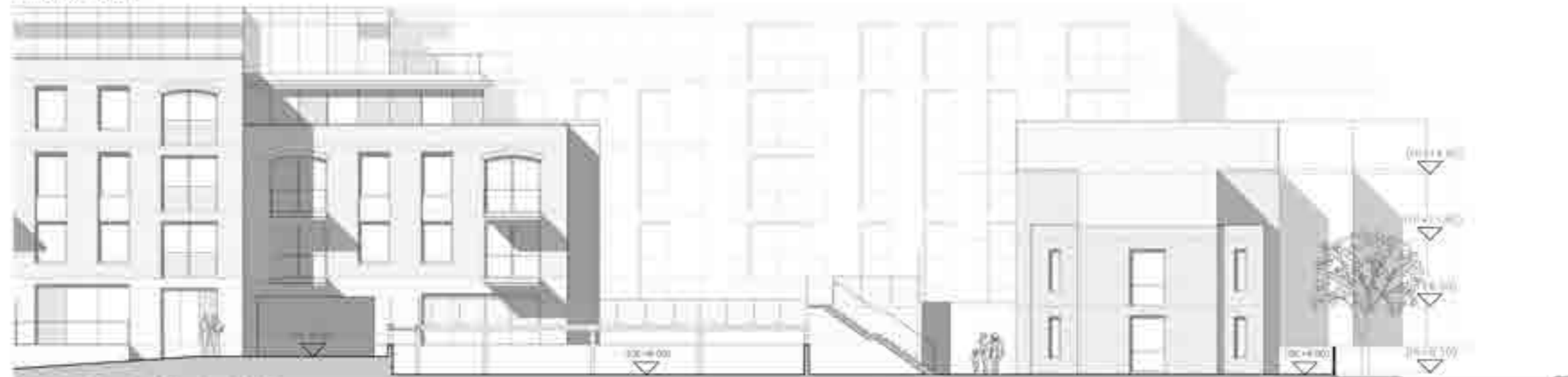
Proposed Elevation 4-4' _detail 1:100
