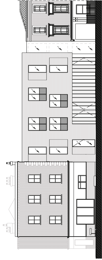
SECTION BB
