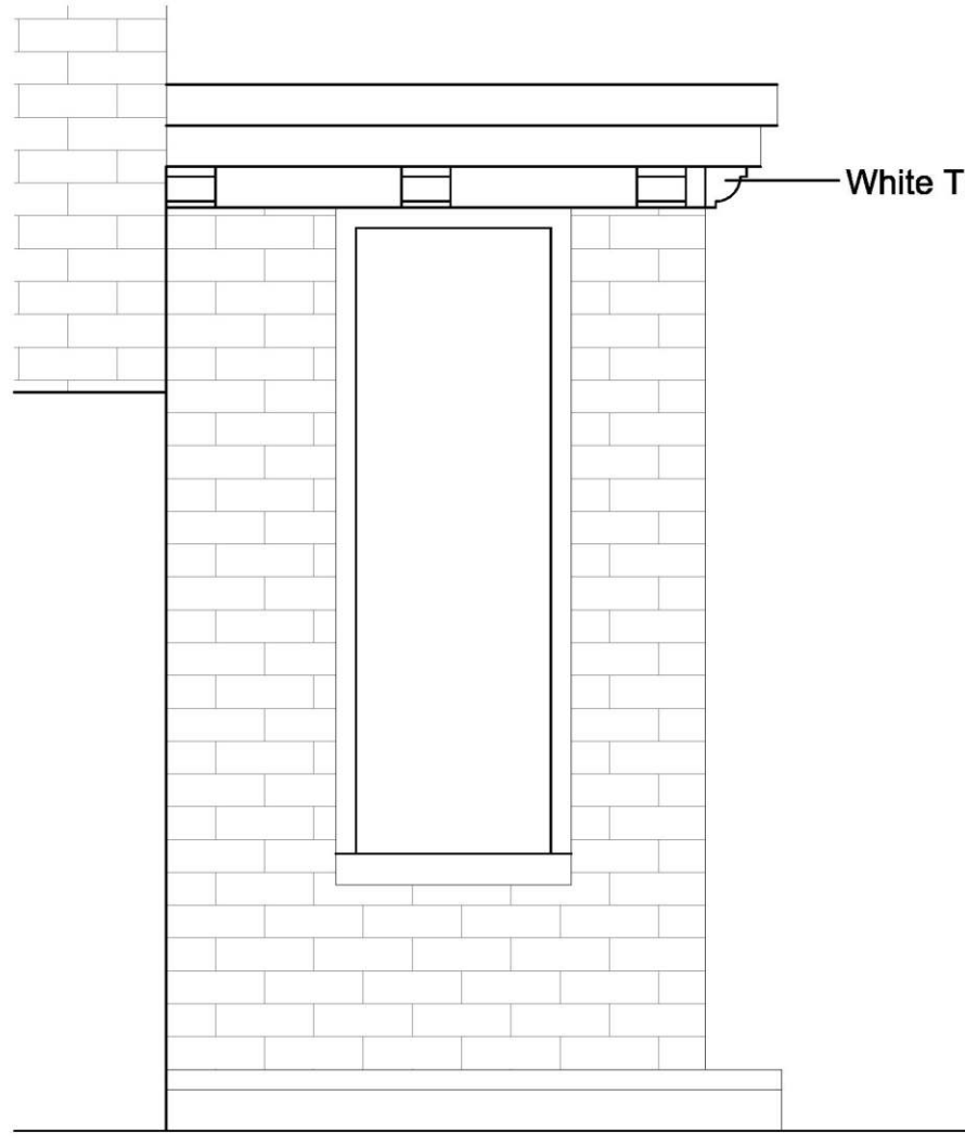
SIDE ELEVATION
