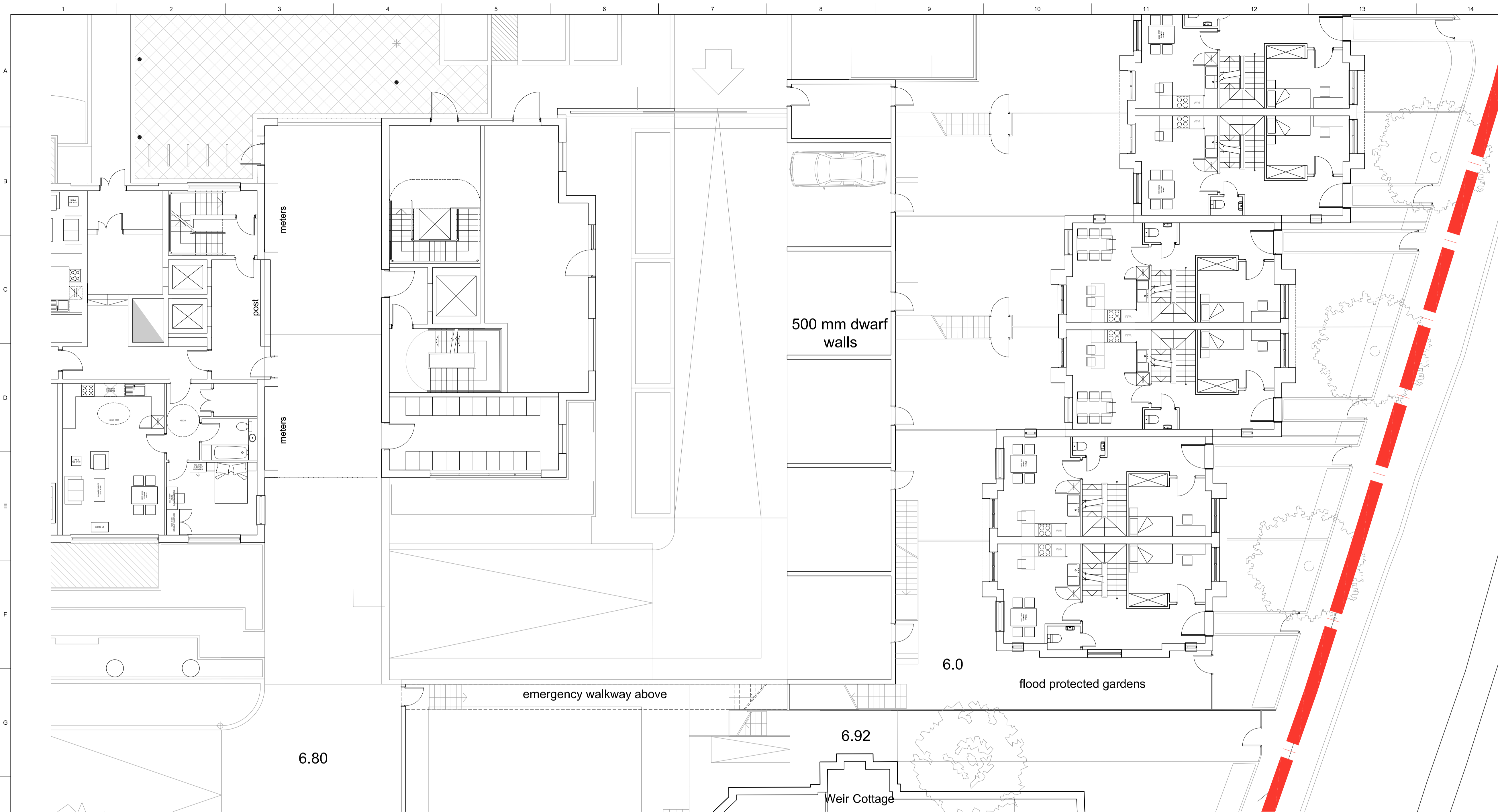
Plan detail 1:100 at level 8.2
