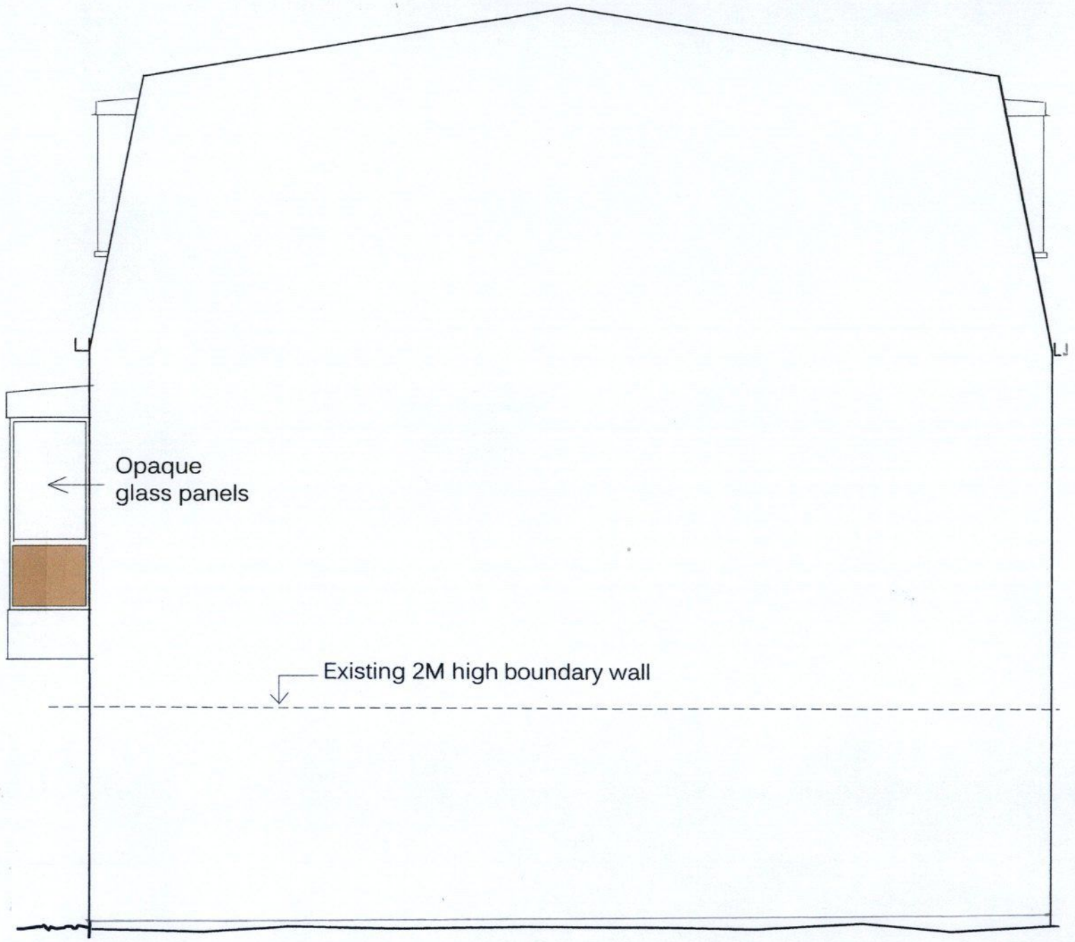
EAST ELEVATION (East and West Elevations Identical)
