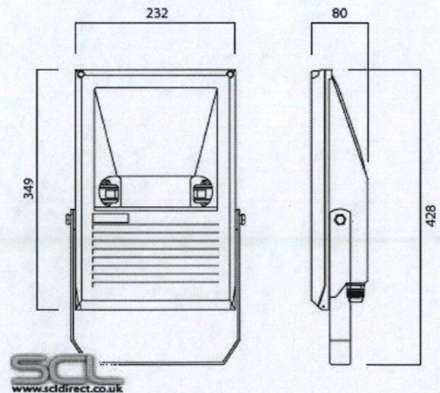
150 Watt Metal Halide IP65 Floodlight Dims
