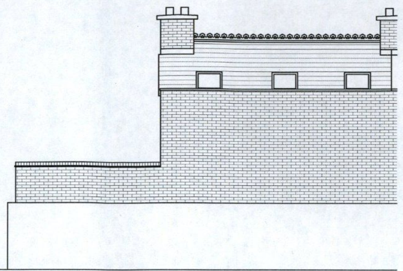
PLOTS 9 - REAR ELEVATION
