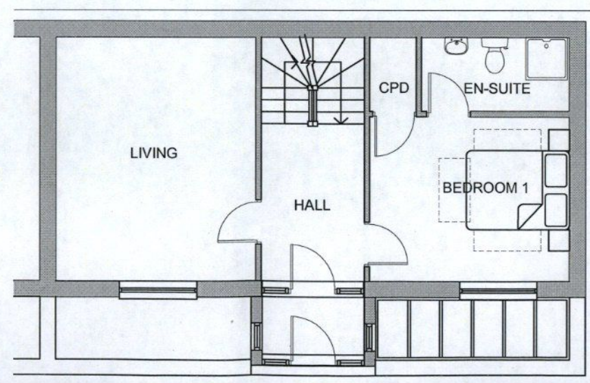
PLOT 9 GROUND FLOOR PLAN
