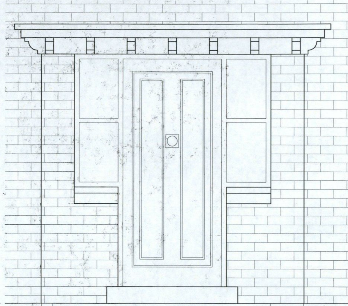
FRONT ELEVATION
