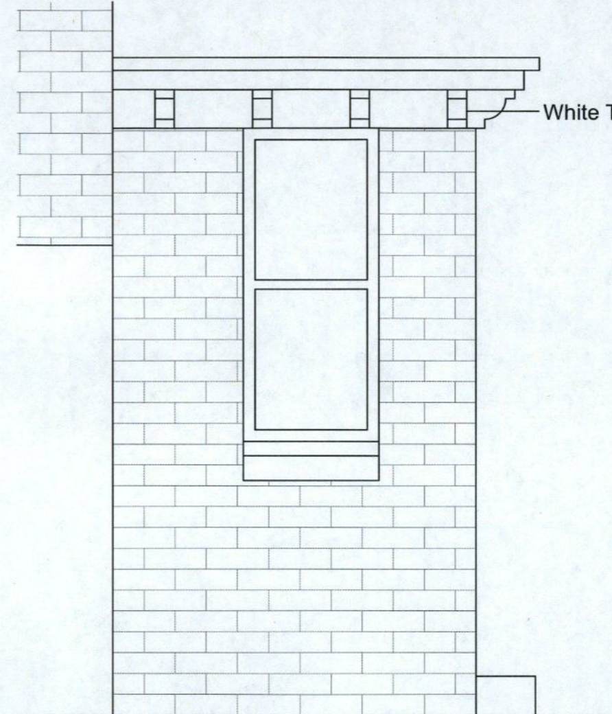
SIDE ELEVATION
