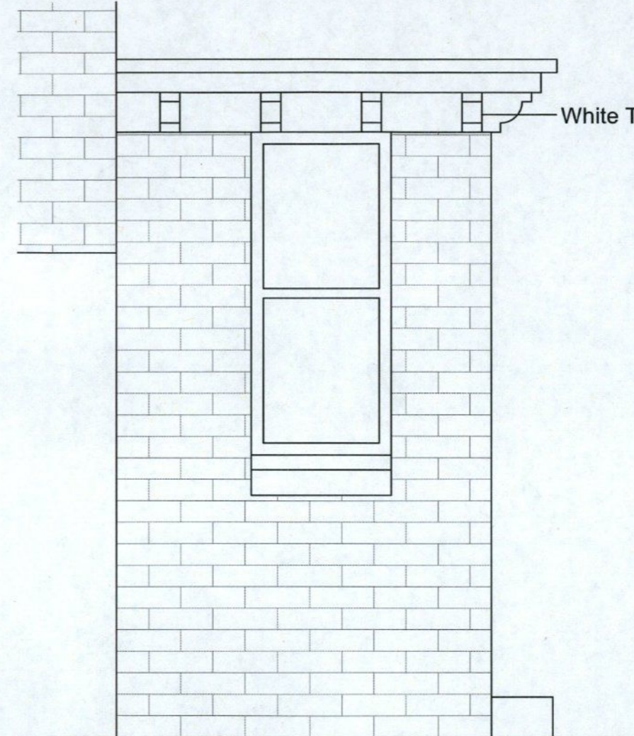
SIDE ELEVATION
