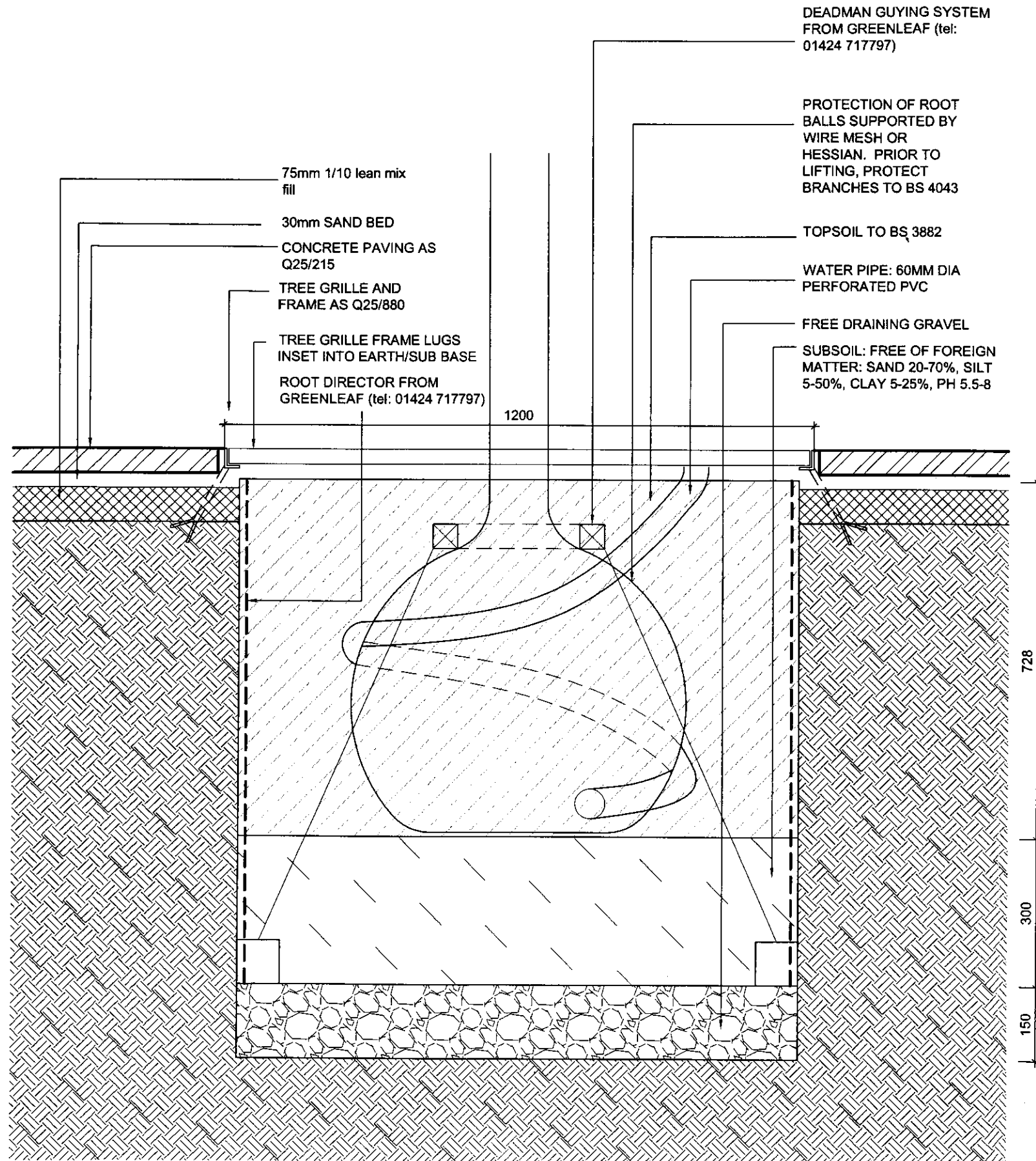
① Paving/ tree pit section
