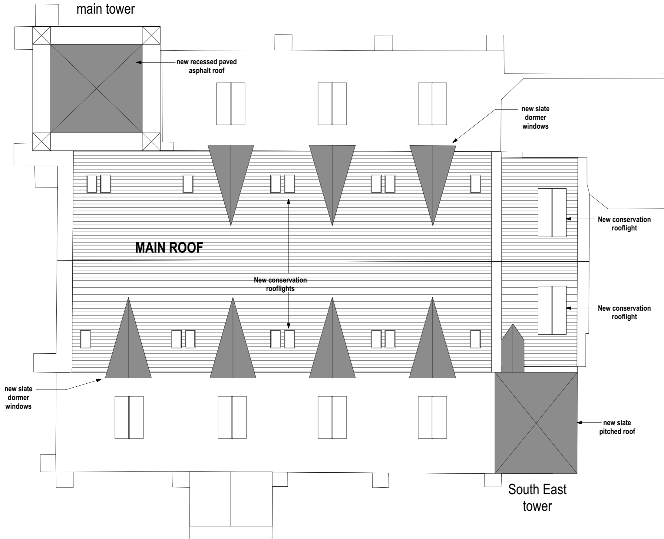
Roof Plan
