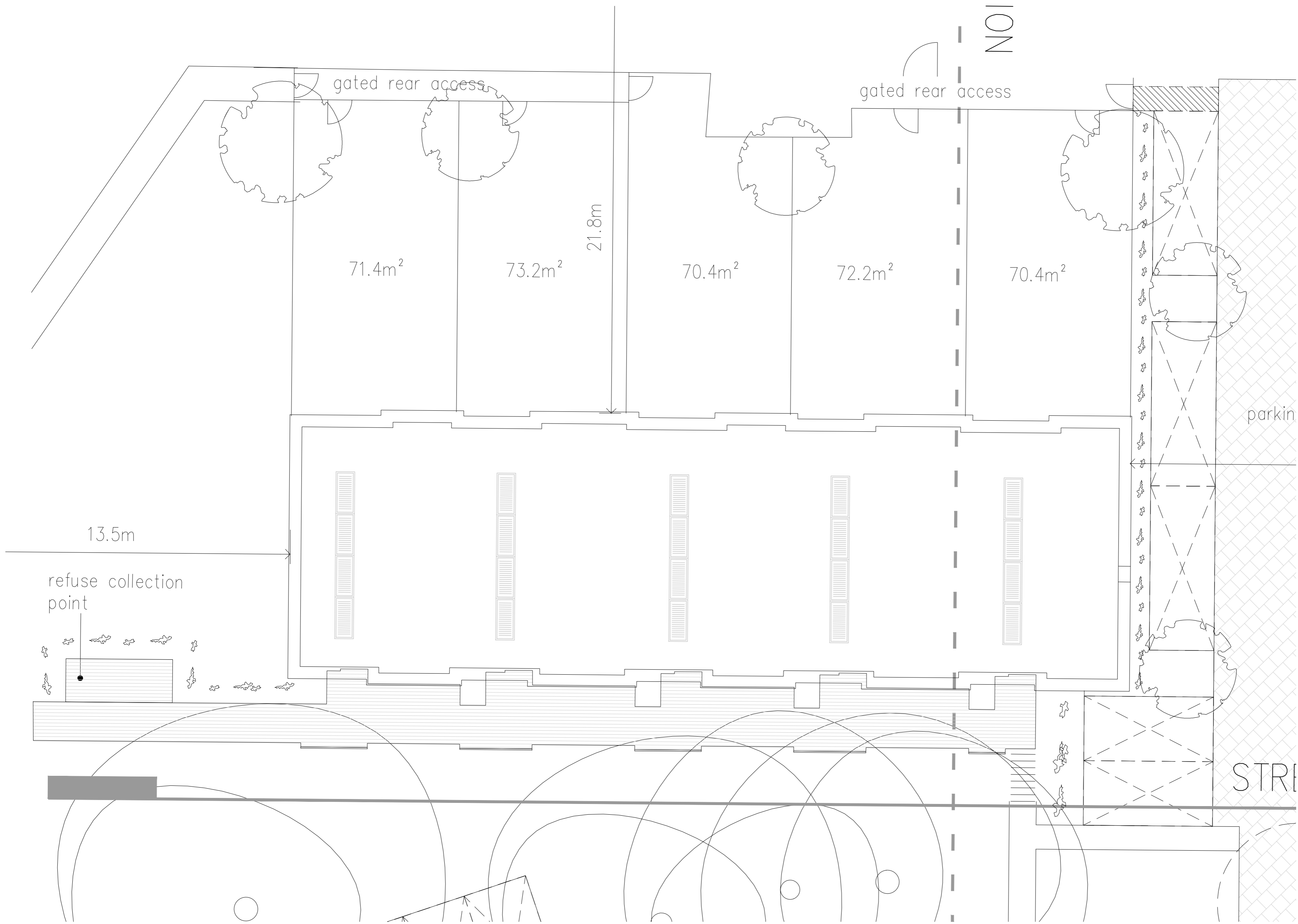
Site A - Ground Floor Plan
