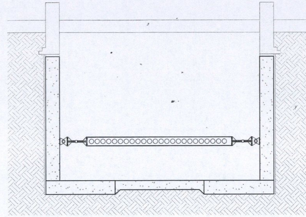
STAGE 8 CAST BASEMENT SLAB AND LET CURE
