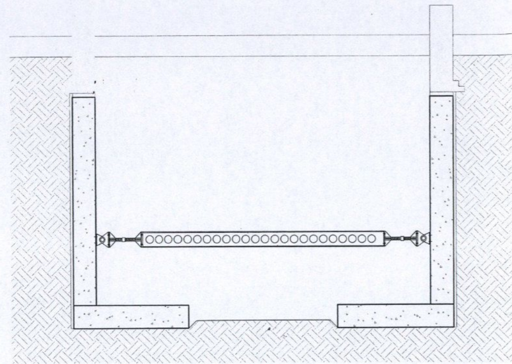
STAGE 7 COMPLETE EXCAVATION TO FORMATION LEVEL
