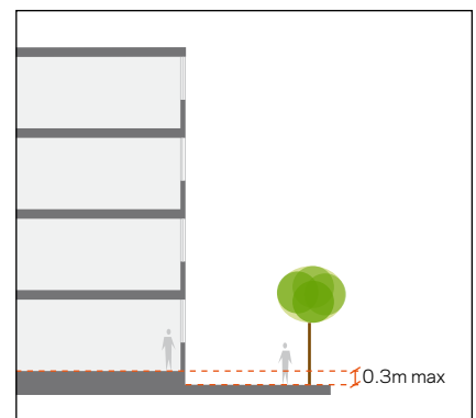
DIAGRAM 5.4.3 GROUND FLOOR LEVELS SHOULD CORRESPOND WITH EXTERNAL LEVELS
