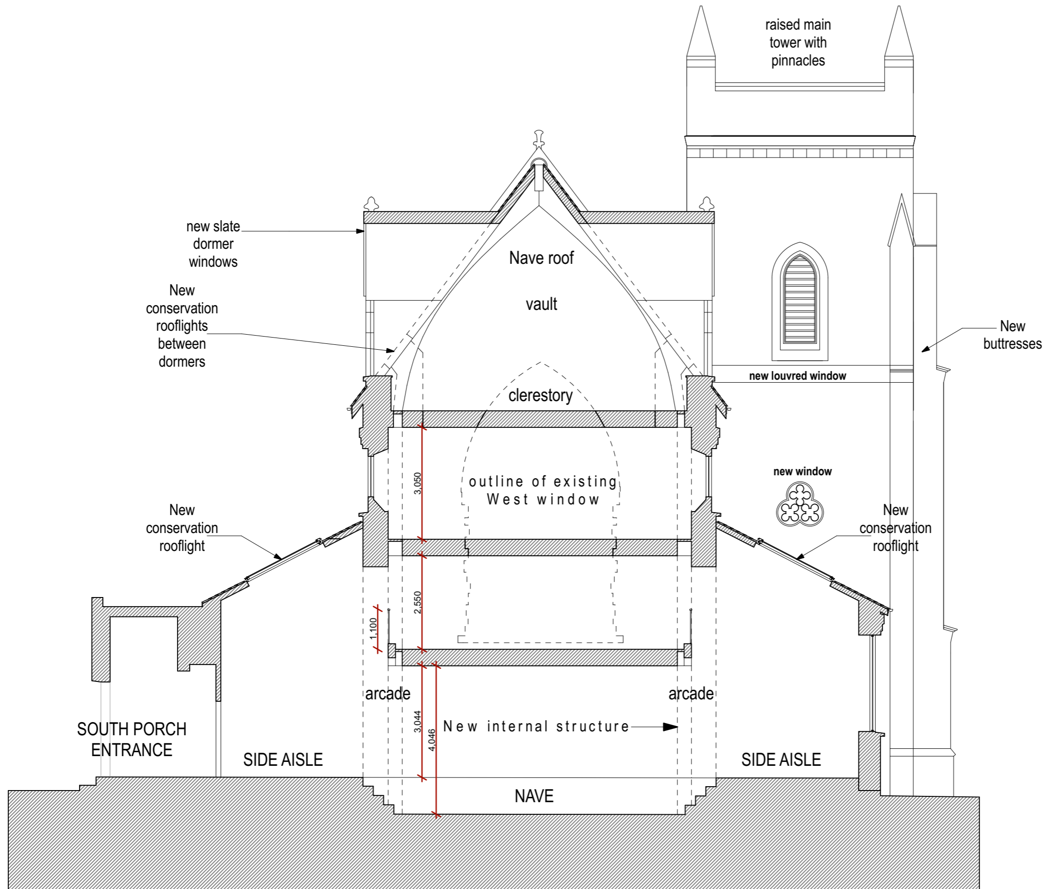
Typical Section
