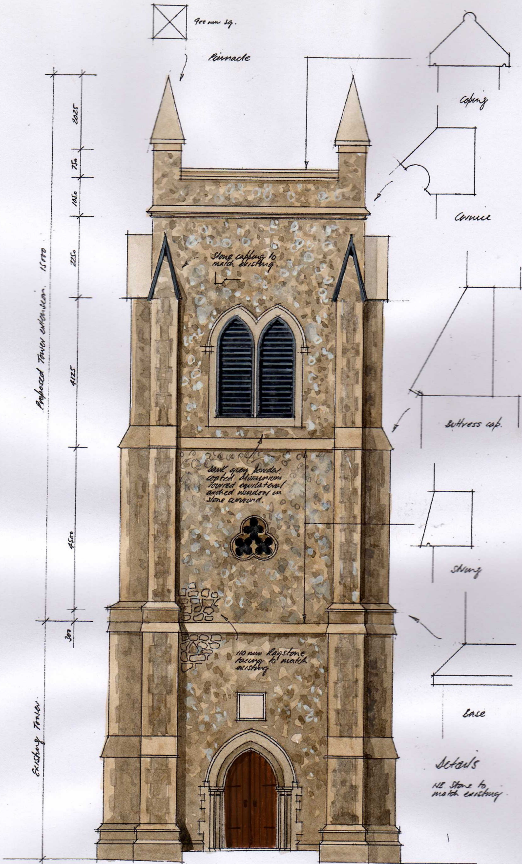
West Elevation Main Tower Christ Church Teddington
