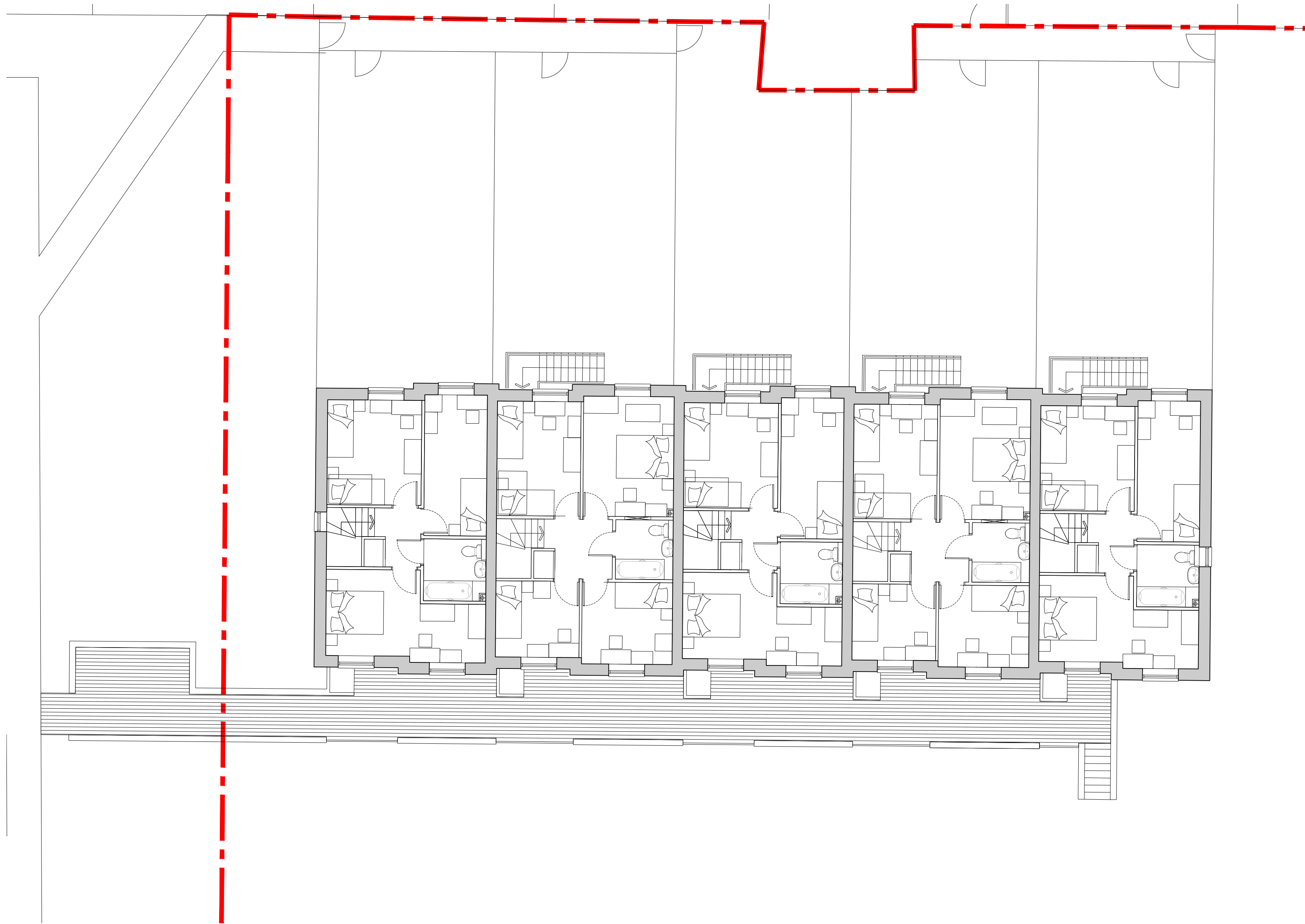
Site A - First Floor Plan
