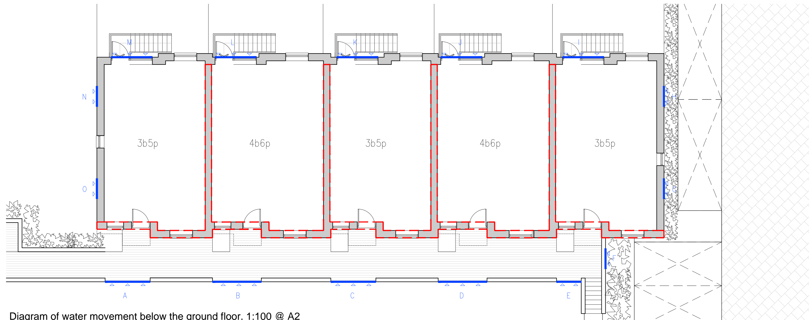
Diagram of water movement below the ground floor. 1:100 @ A2
