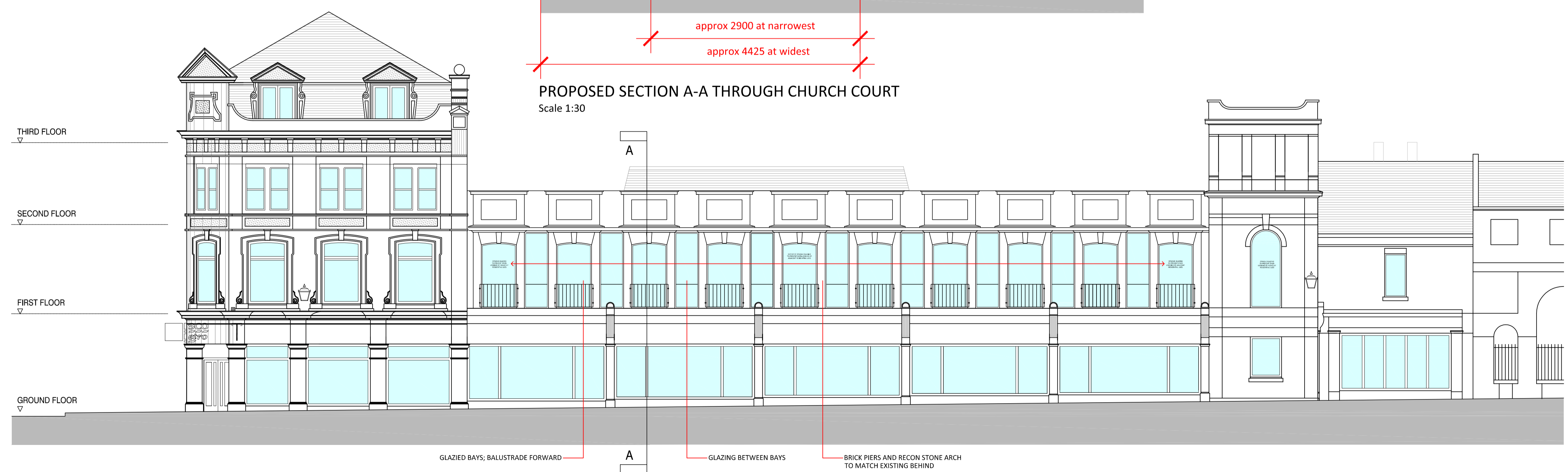
PROPOSED CHURCH COURT ELEVATION Scale 1:100
