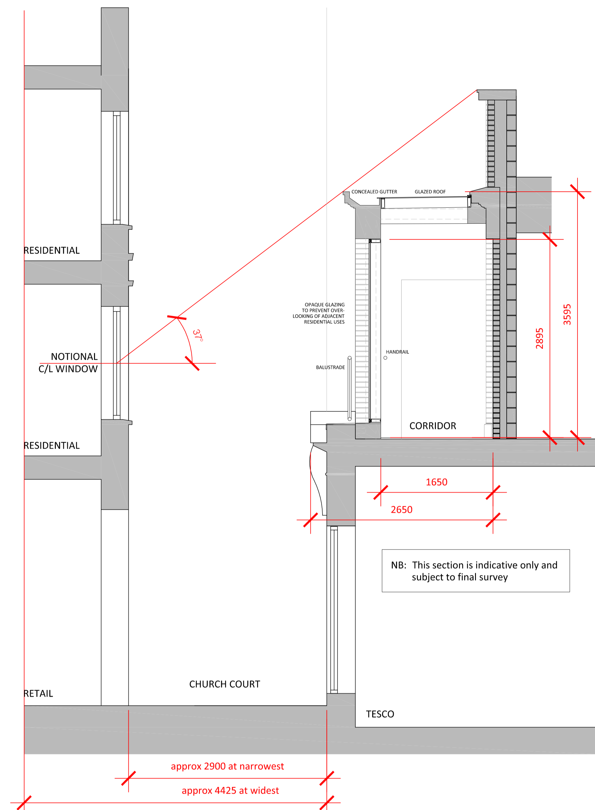
PROPOSED SECTION A-A THROUGH CHURCH COURT Scale 1:30
