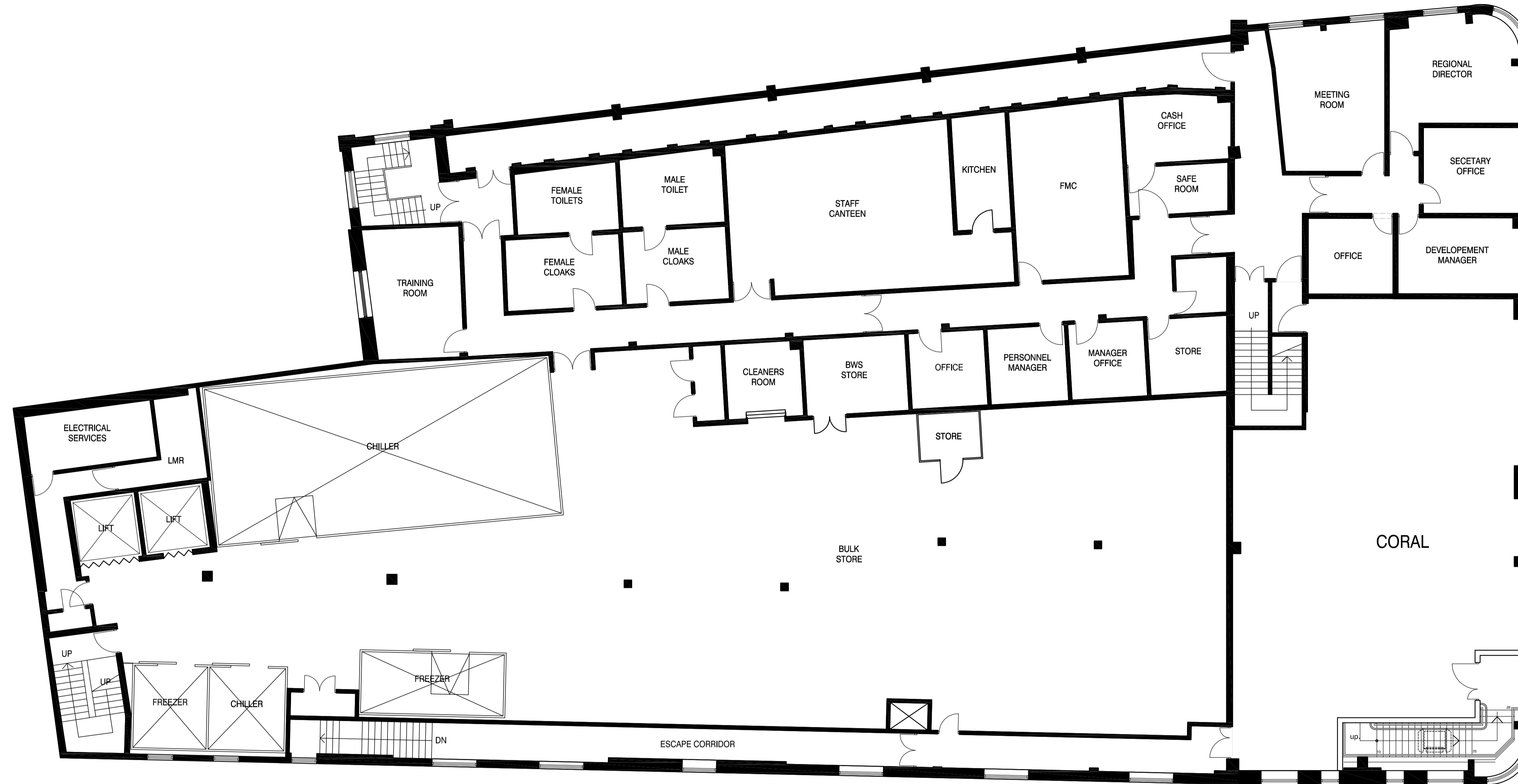
PROPOSED FIRST FLOOR
