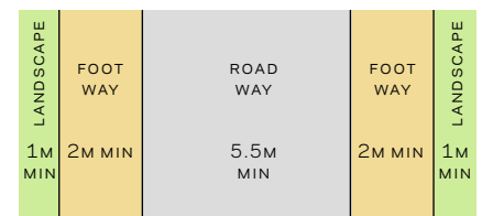
DIAGRAM 3.4.5 RIGHT-OF-WAY LAYOUT
