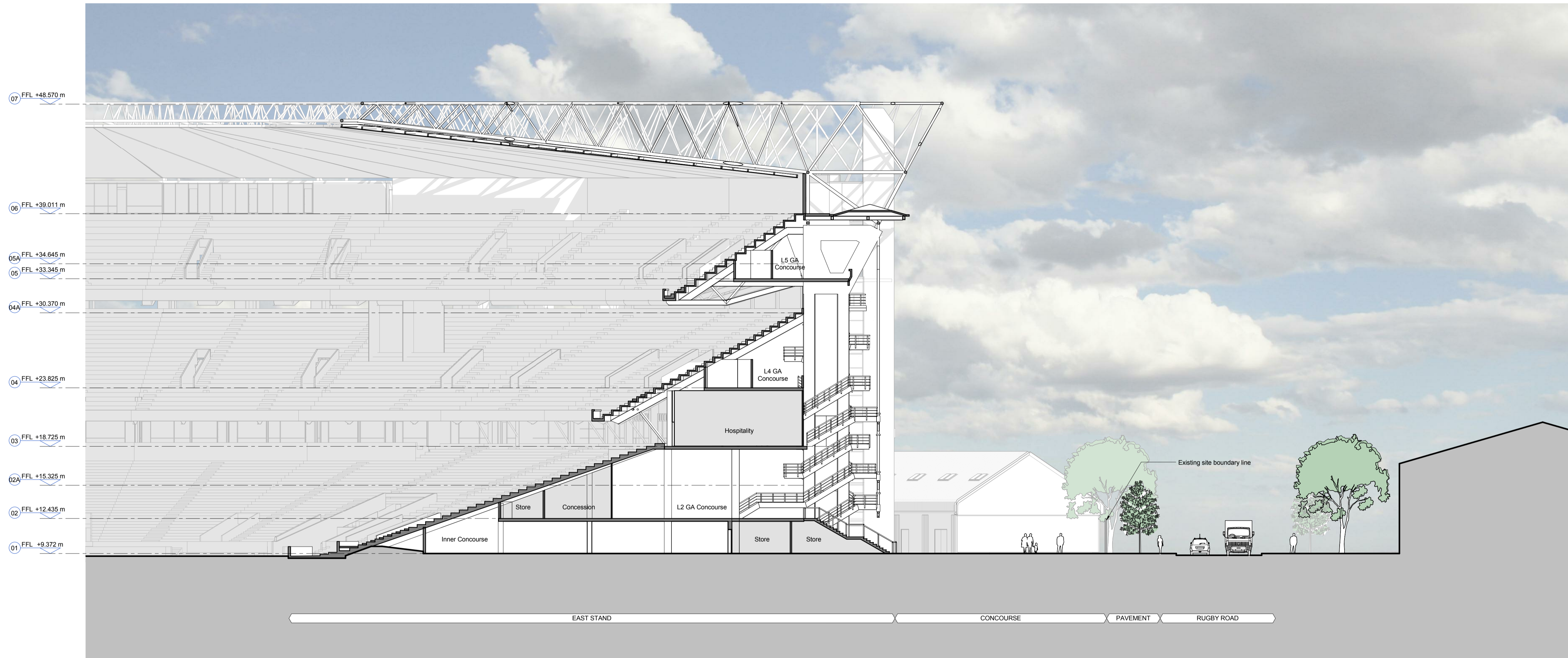
1 SECTION C SECTION EXISTING 1 : 200
