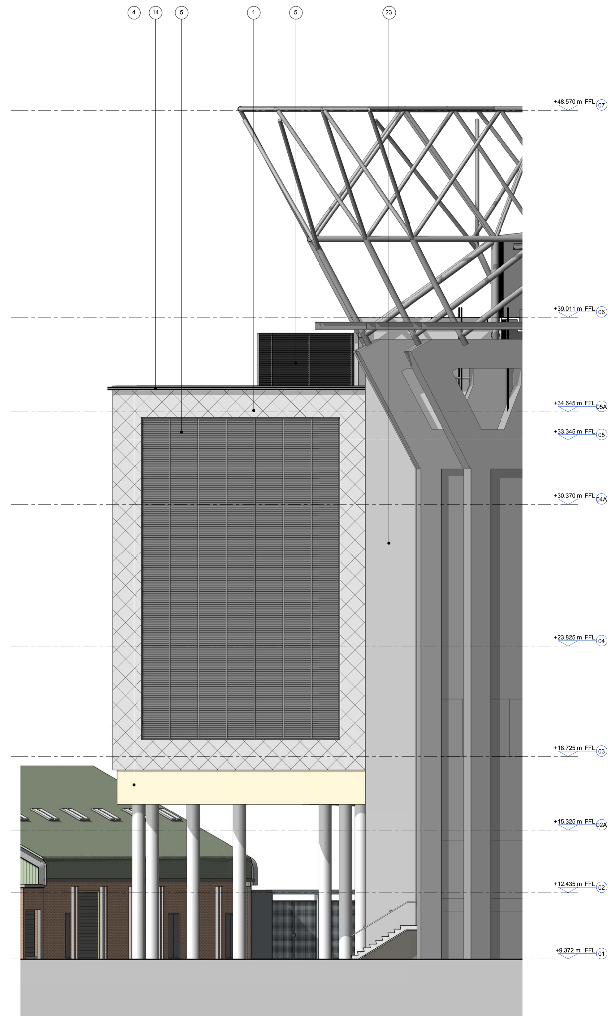
2 ELEVATION NORTH DETAILED ELEVATION 1:100
