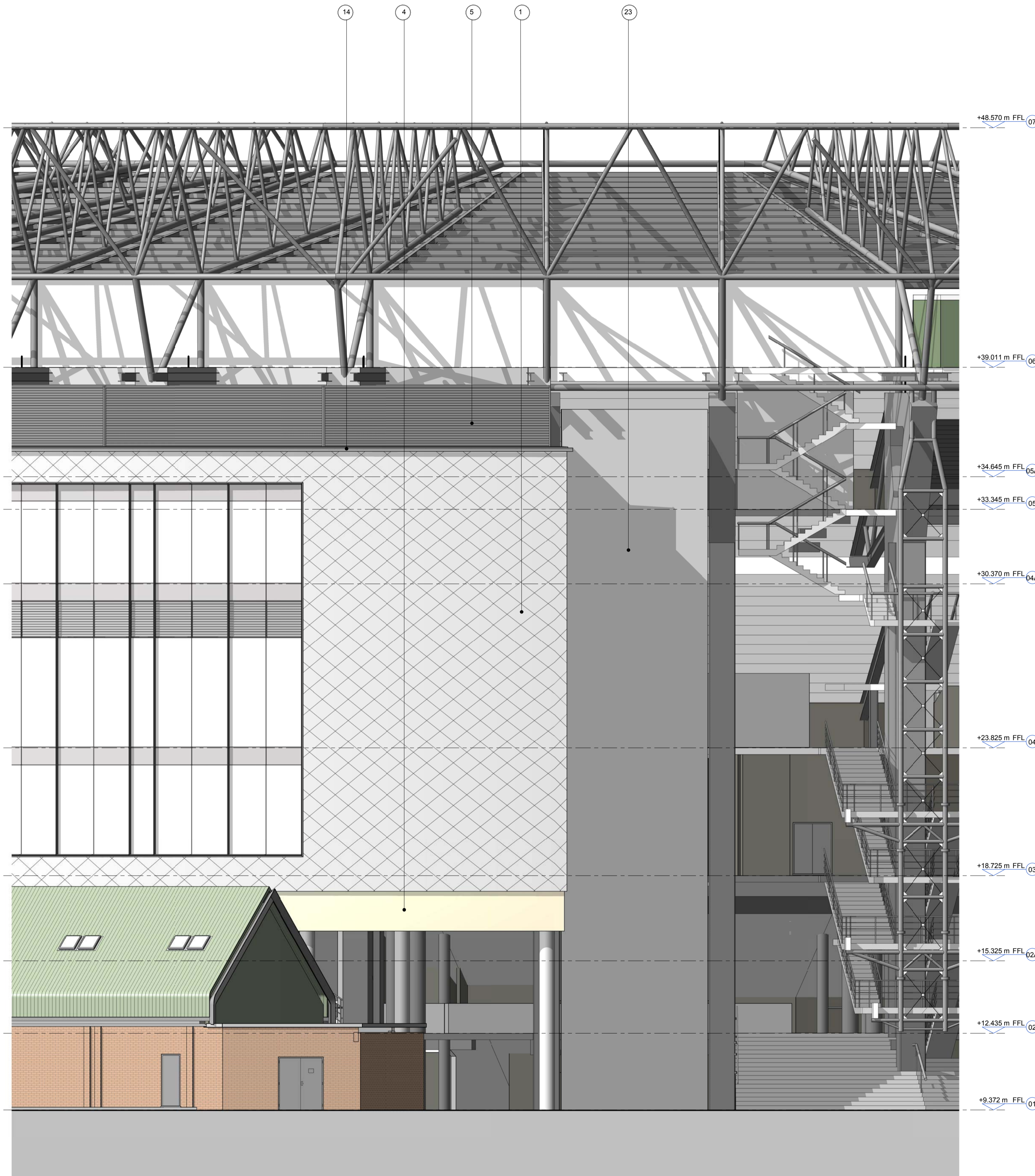
1 ELEVATION NORTH EAST DETAILED ELEVATION 1:100
