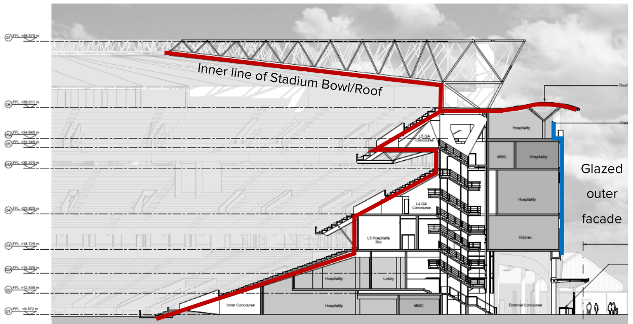
Figure 2 Cross-section through East Stand (Proposed)
