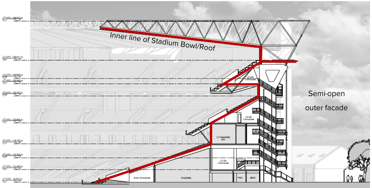
Figure 2 Cross-section through East Stand (Proposed)
