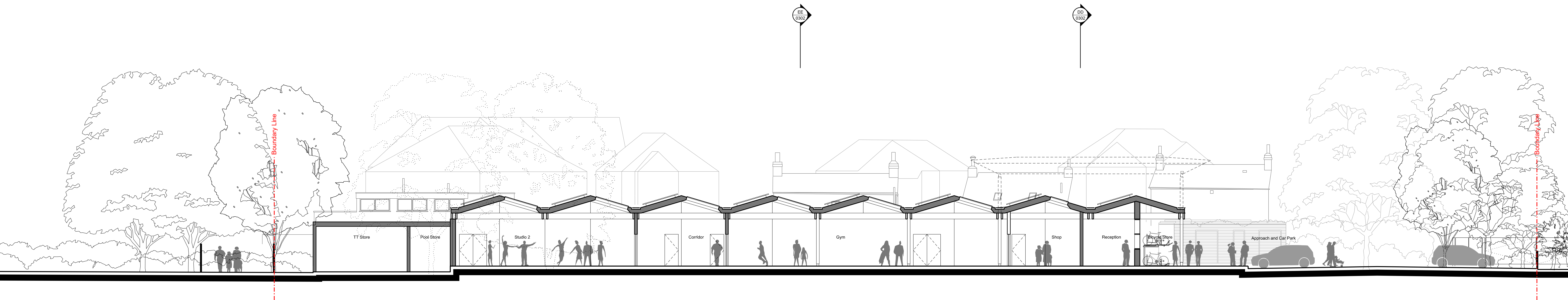
03 SEC Proposed Section C - C 1:100@A0
