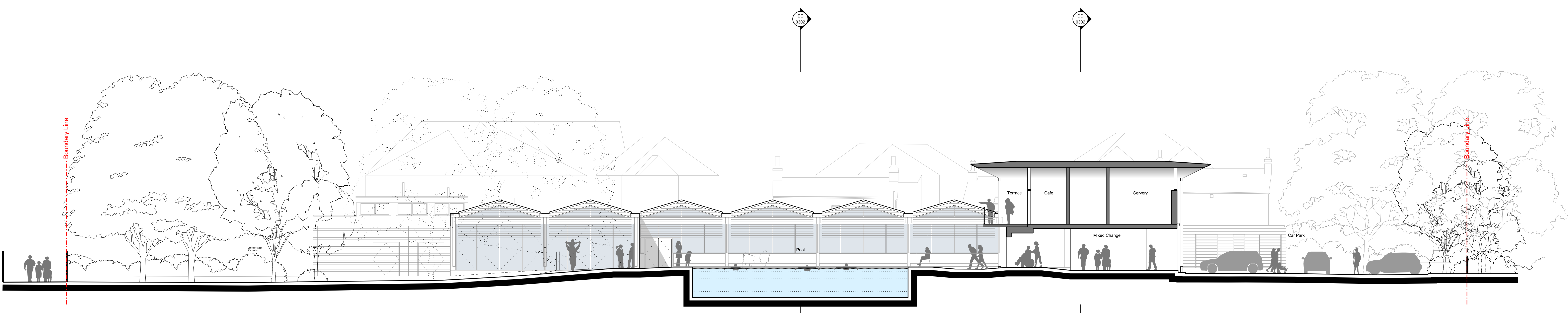
01 SEC Proposed Section A - A 1:100@A0
