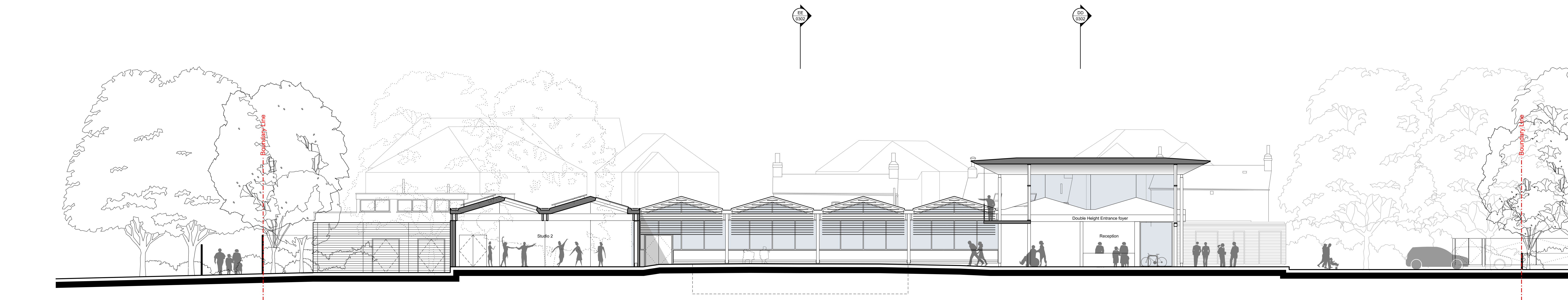
02 SEC Proposed Section B - B 1:100@A0
