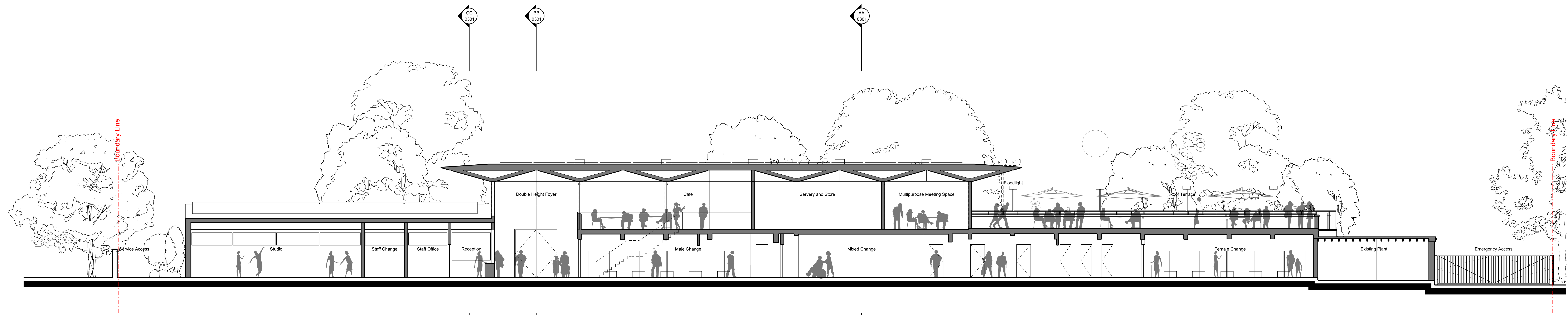
01 SEC Proposed Section D - D 1:100@A0
