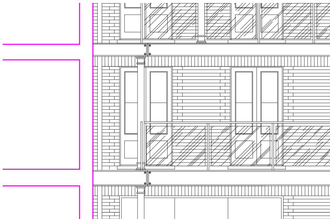
DETAIL @ 1.50
