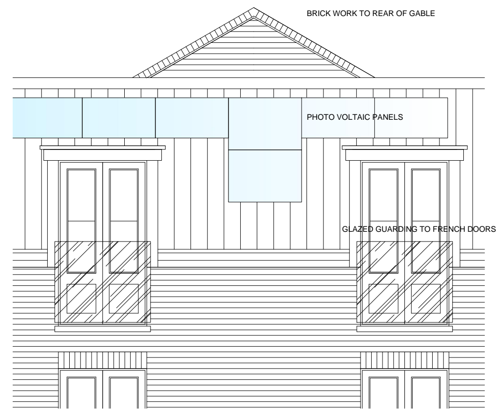
DETAIL @ 1.50
