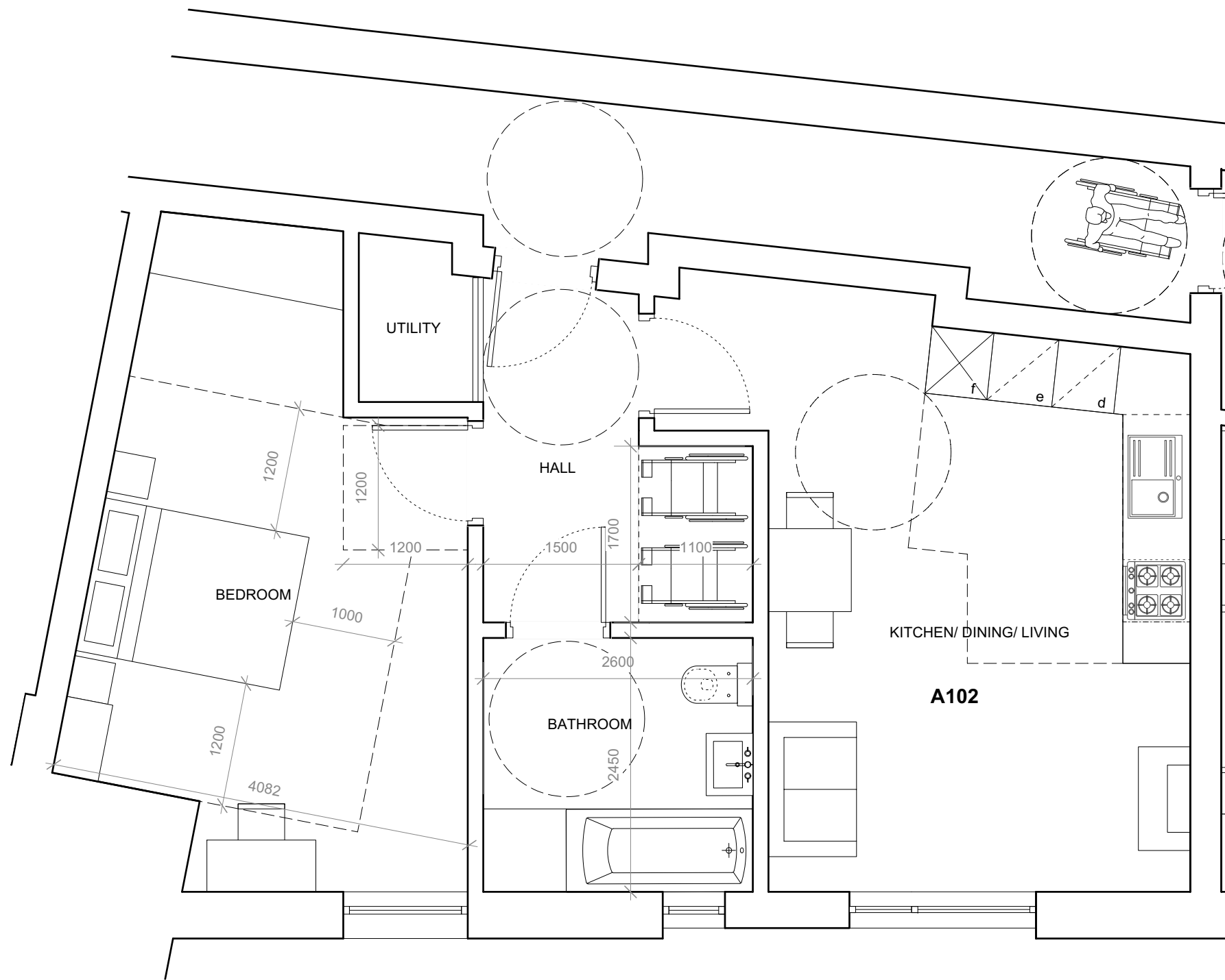
PROPOSED WHEELCHAIR ADAPTABLE UNIT A102 1 BED 2 PERSON APARTMENT
