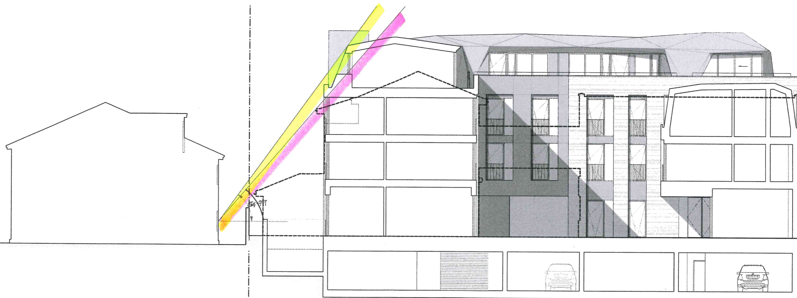
PROPOSED ELEVATION SECTION H - COURTYARD EAST ELEVATION
