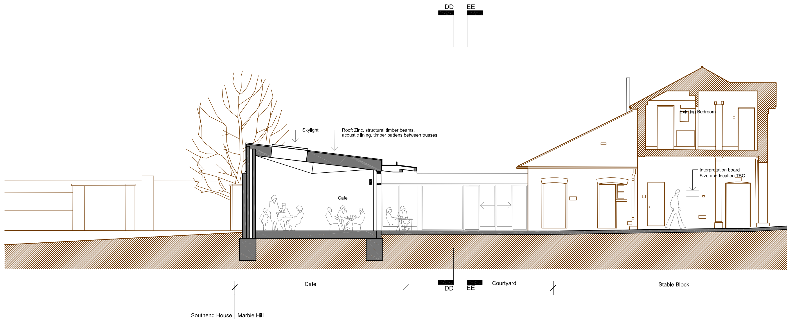
Section BB
