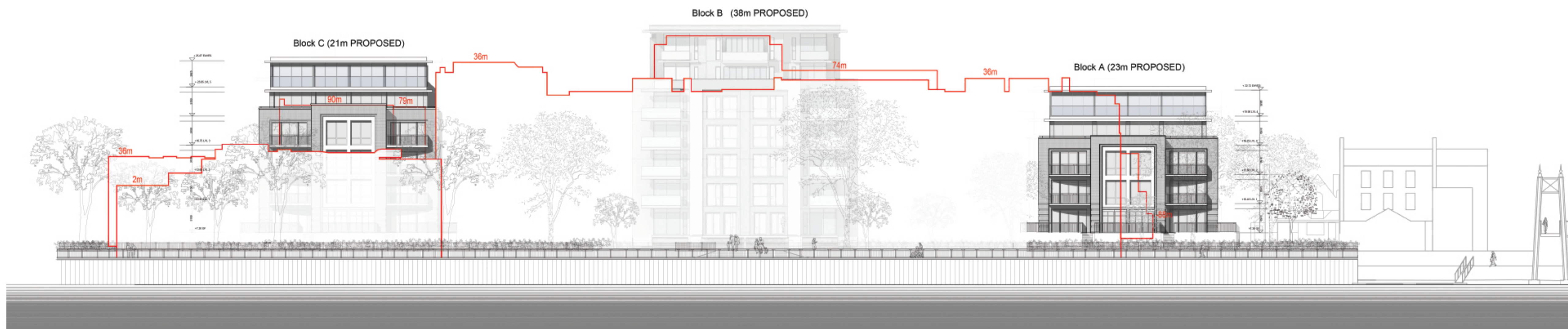
Proposed Elevation 2-2' (Dimensions noted are from the relevant boundary plane)
