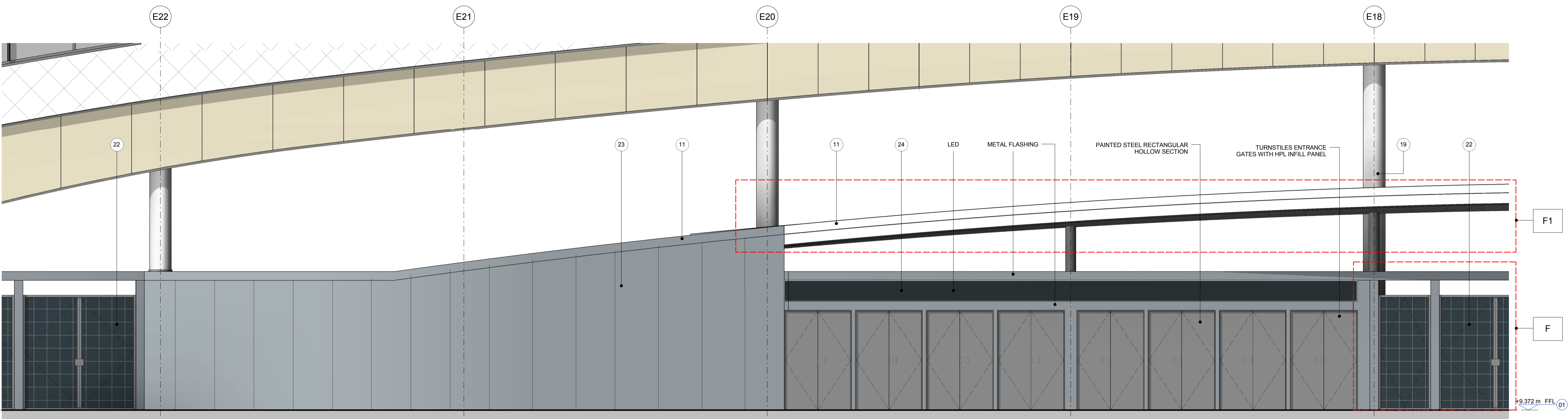
1 ELEVATION STREET FRONTAGE DETAILED ELEVATION 2 1:50
