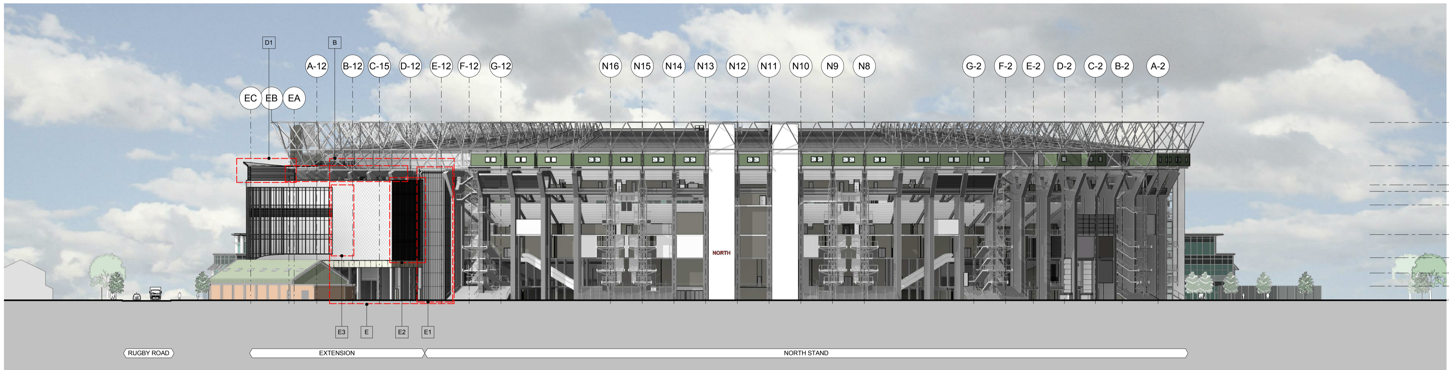
1 ELEVATION LEVEL 1 GA - PROPOSED LANDSCAPING 1 : 500
