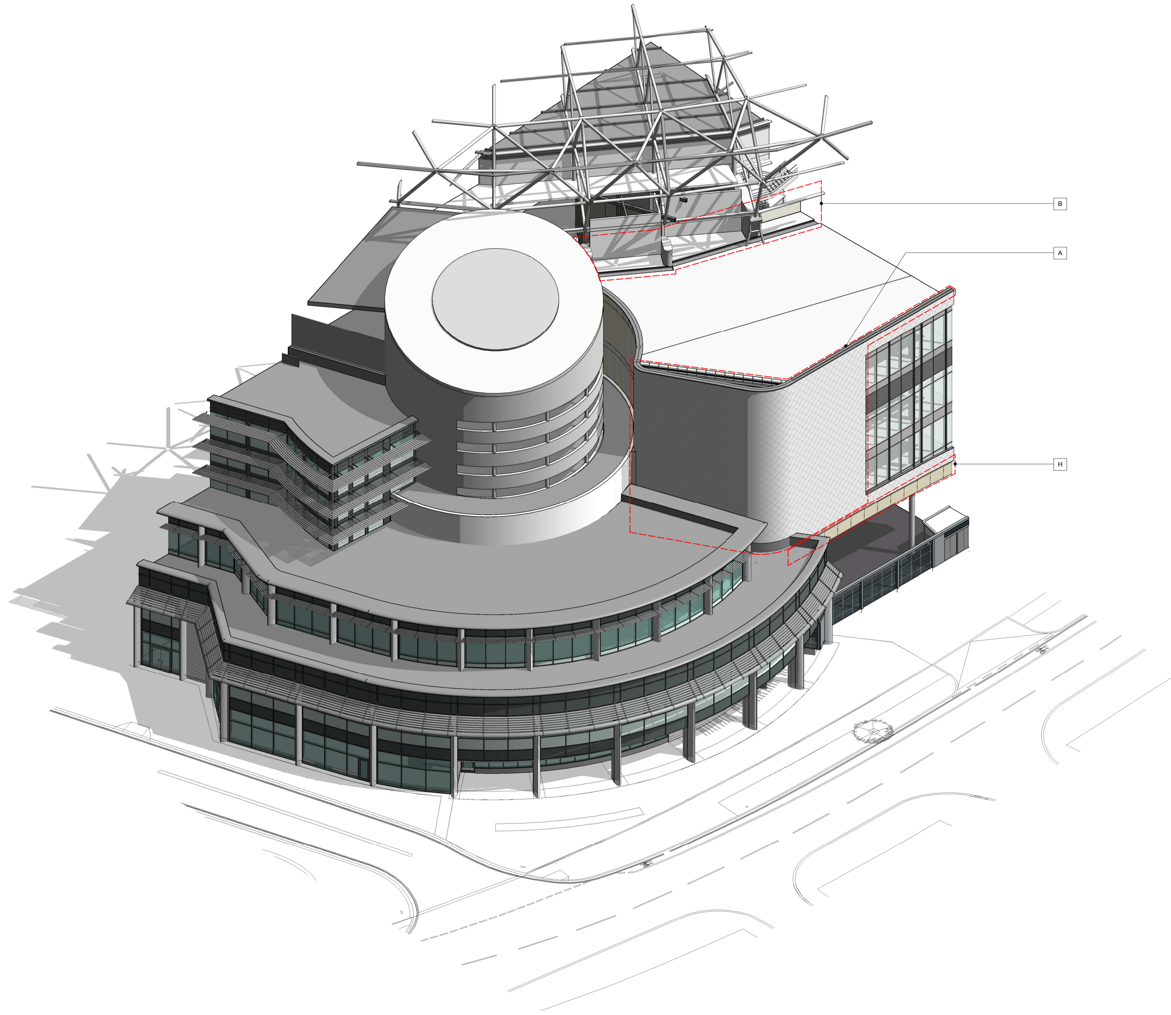
1 3D VIEW AXONOMETRIC VIEW FROM SOUTH EAST SHOWING THE NEW STAND EXTENSION MEETING EXISTING SOUTH STAND
